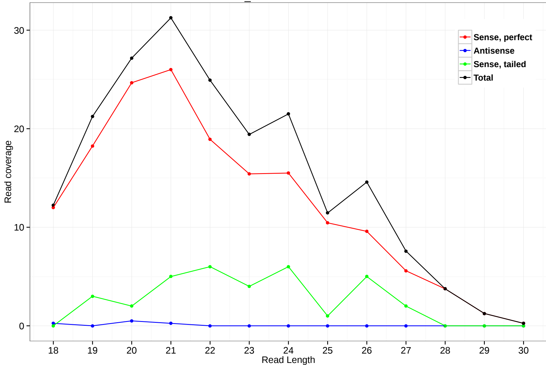
scaffold_4820:2260549-2260868
