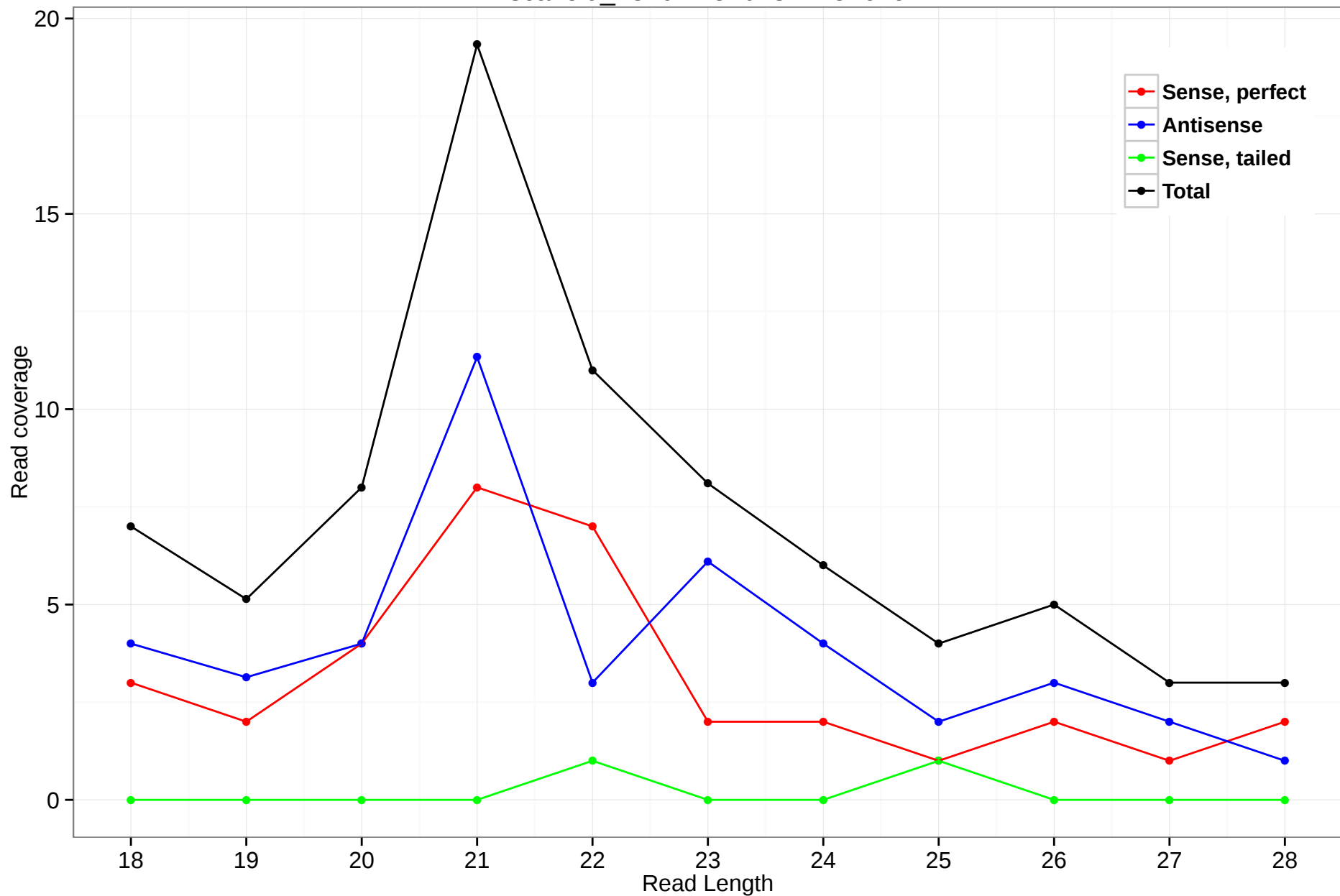
scaffold_4820:2251048-2251629
