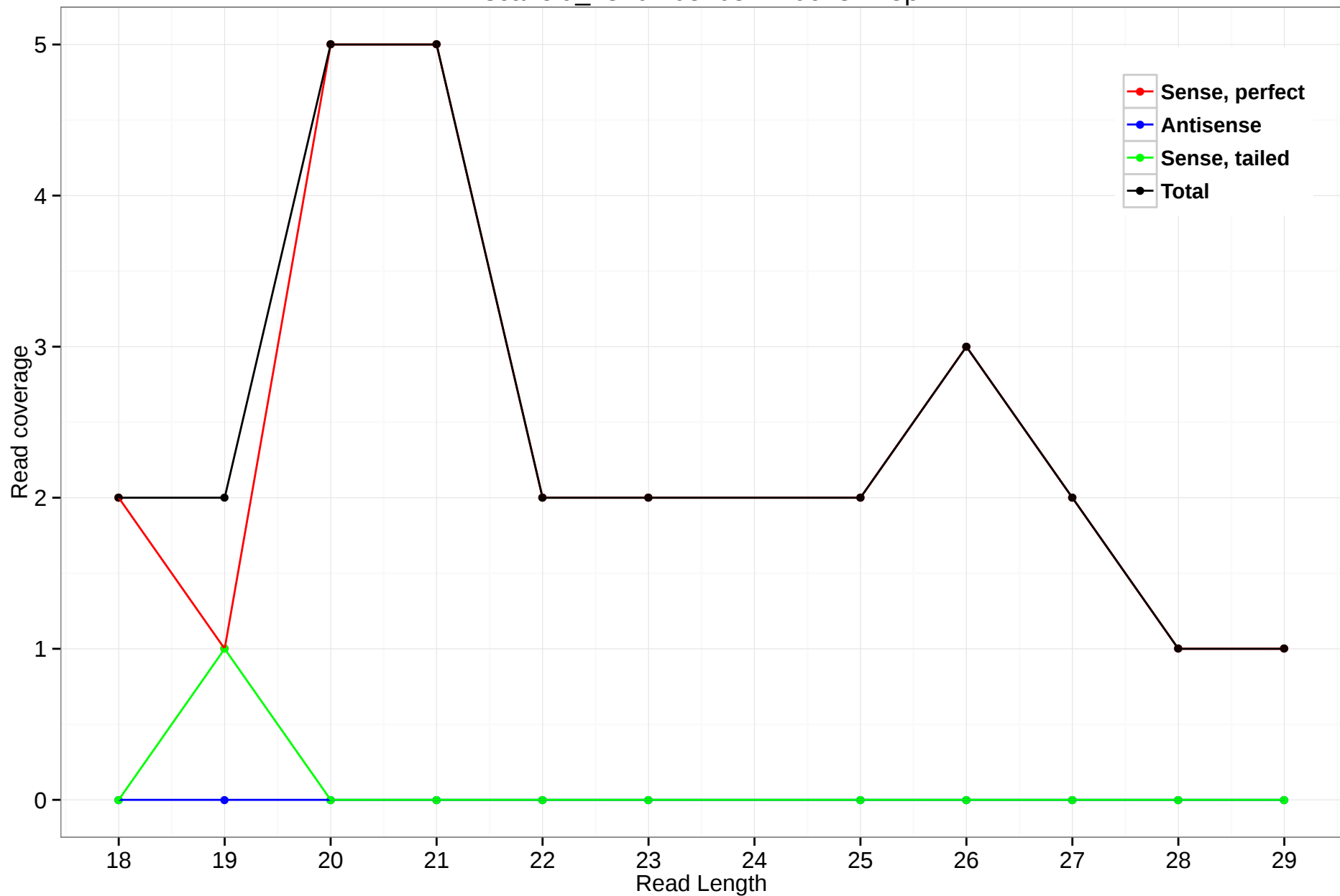
scaffold_4820:2054051-2061871.5p
