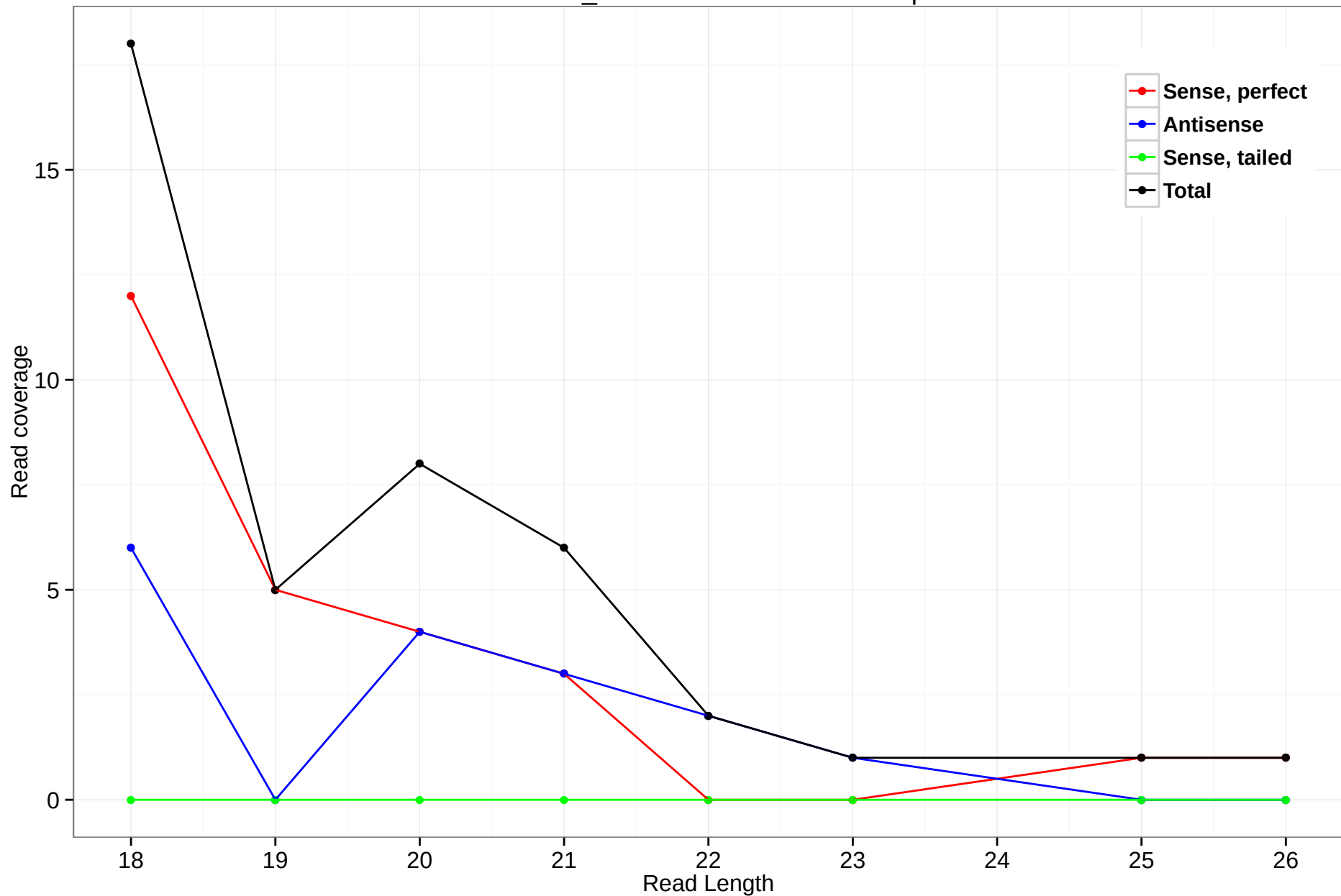
scaffold_4784:9823989-9825000.3p
