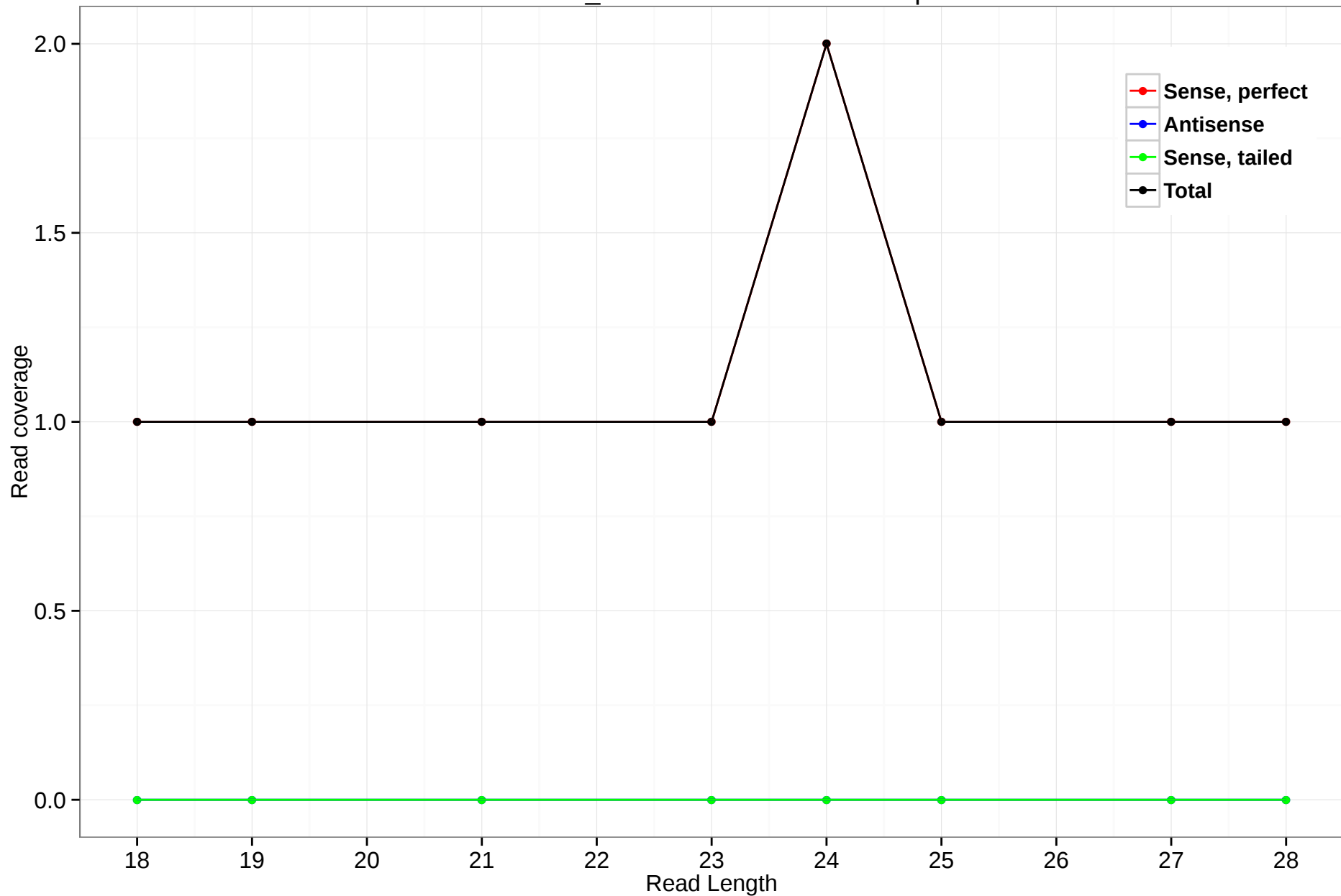
scaffold_4784:9709189-9710042.5p
