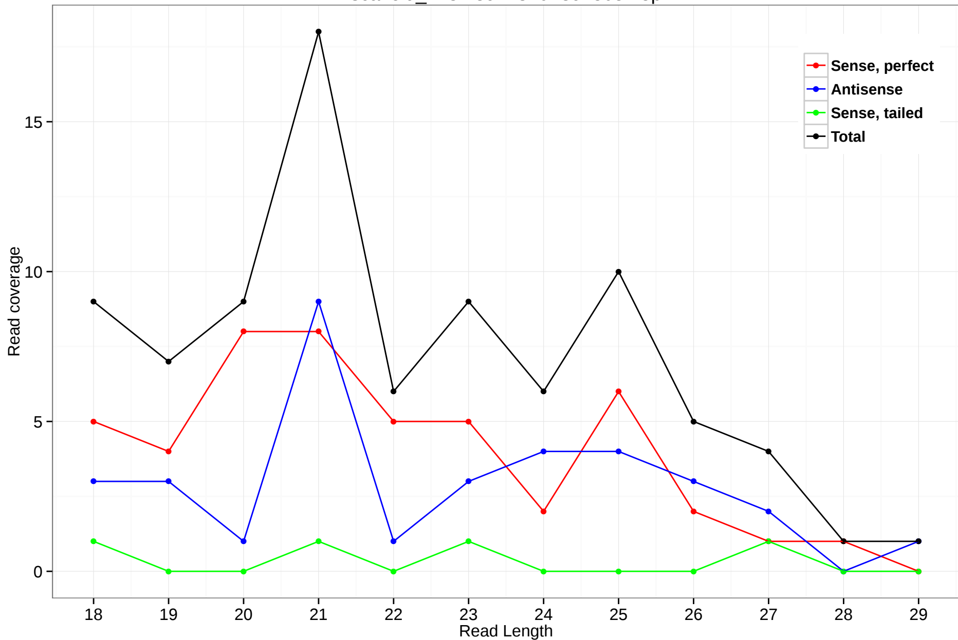
scaffold_4784:8924310-8925051.5p
