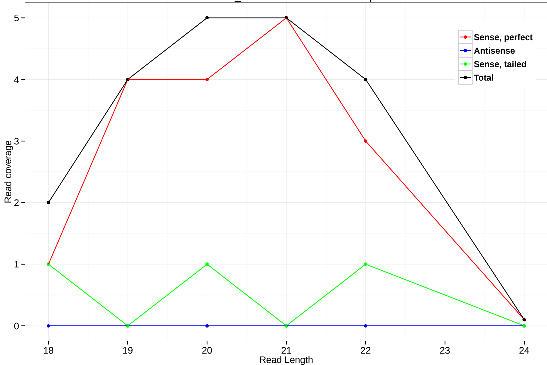
scaffold_4784:8390445-8400195.3p
