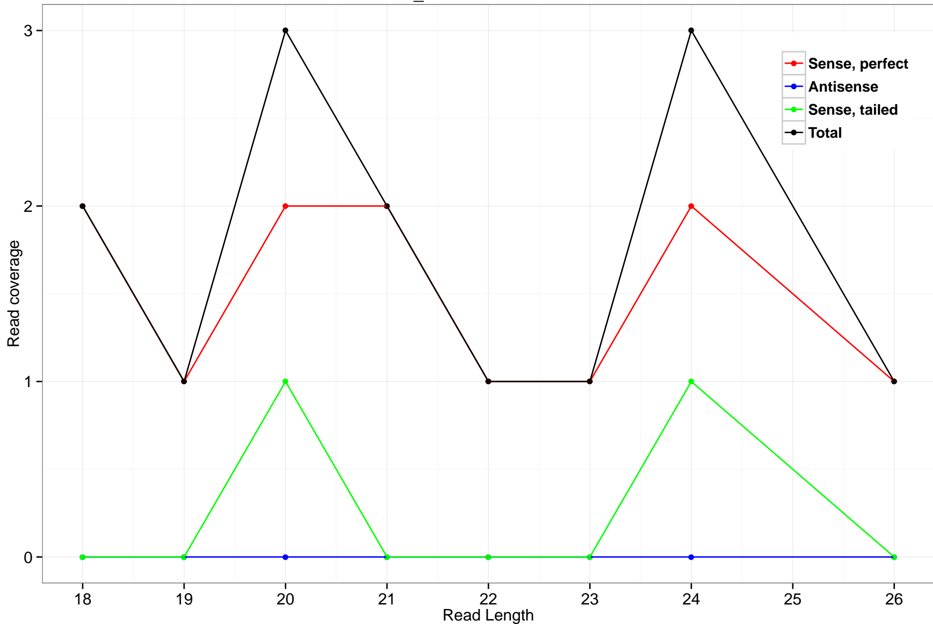
scaffold_4784:7044496-7044661
