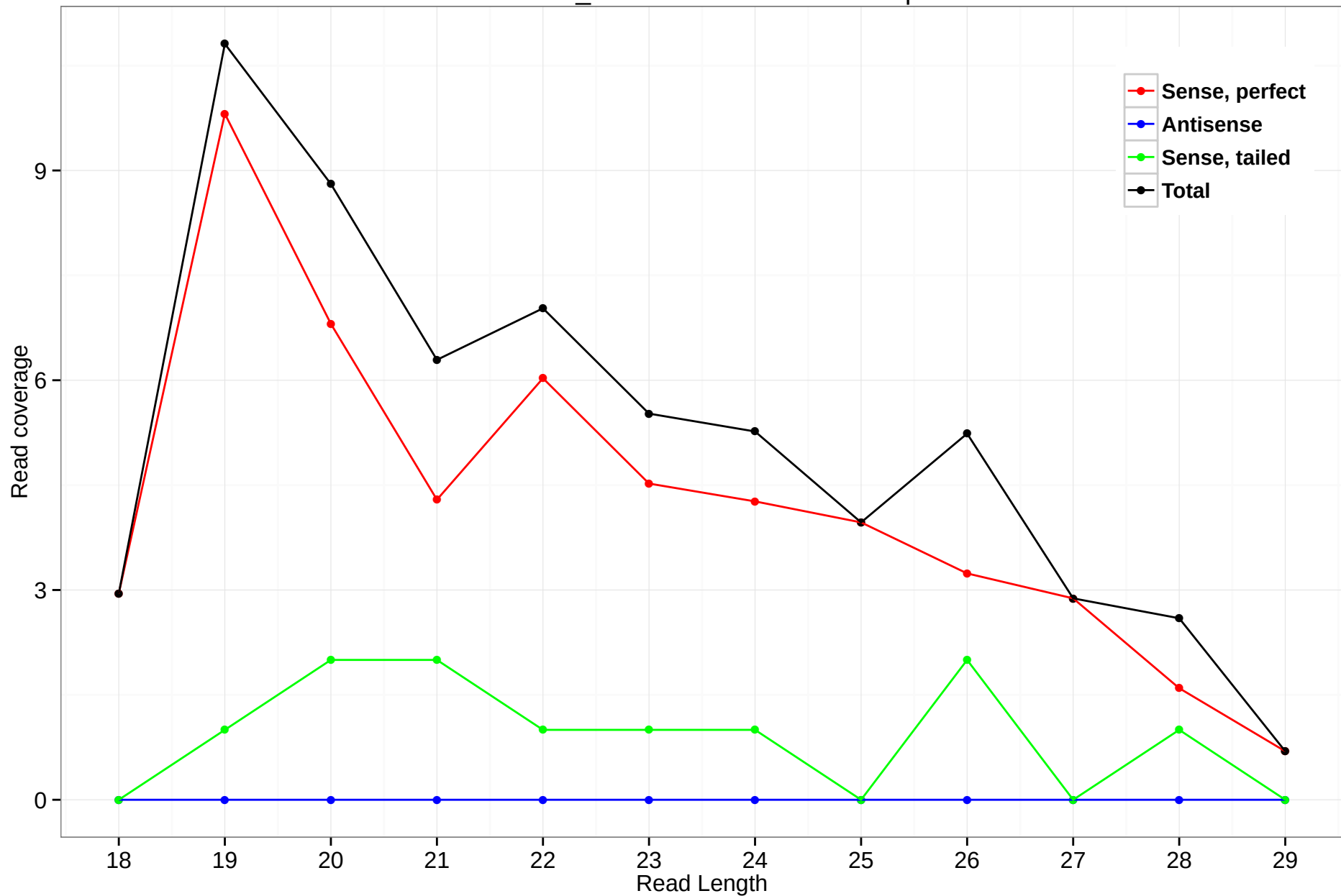
scaffold_4784:6598509-6601117.3p
