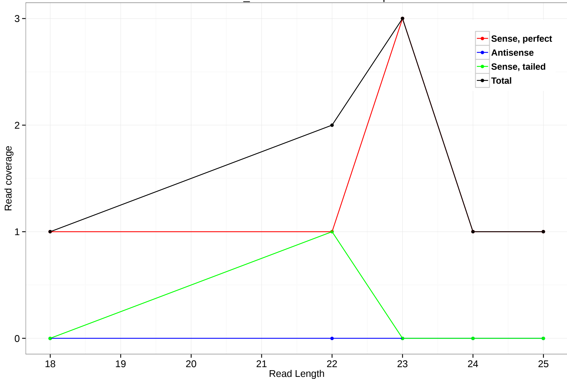
scaffold_4784:3532444-3538223.5p
