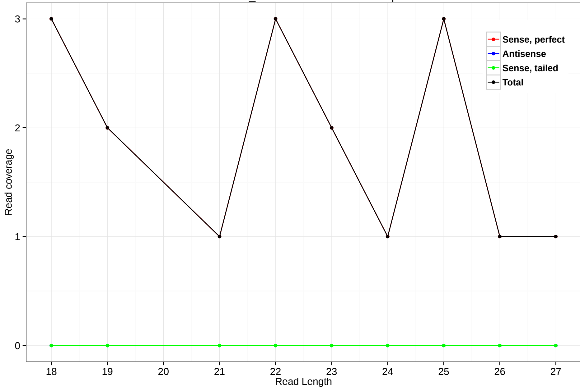
scaffold_4784:3503090-3503725.5p
