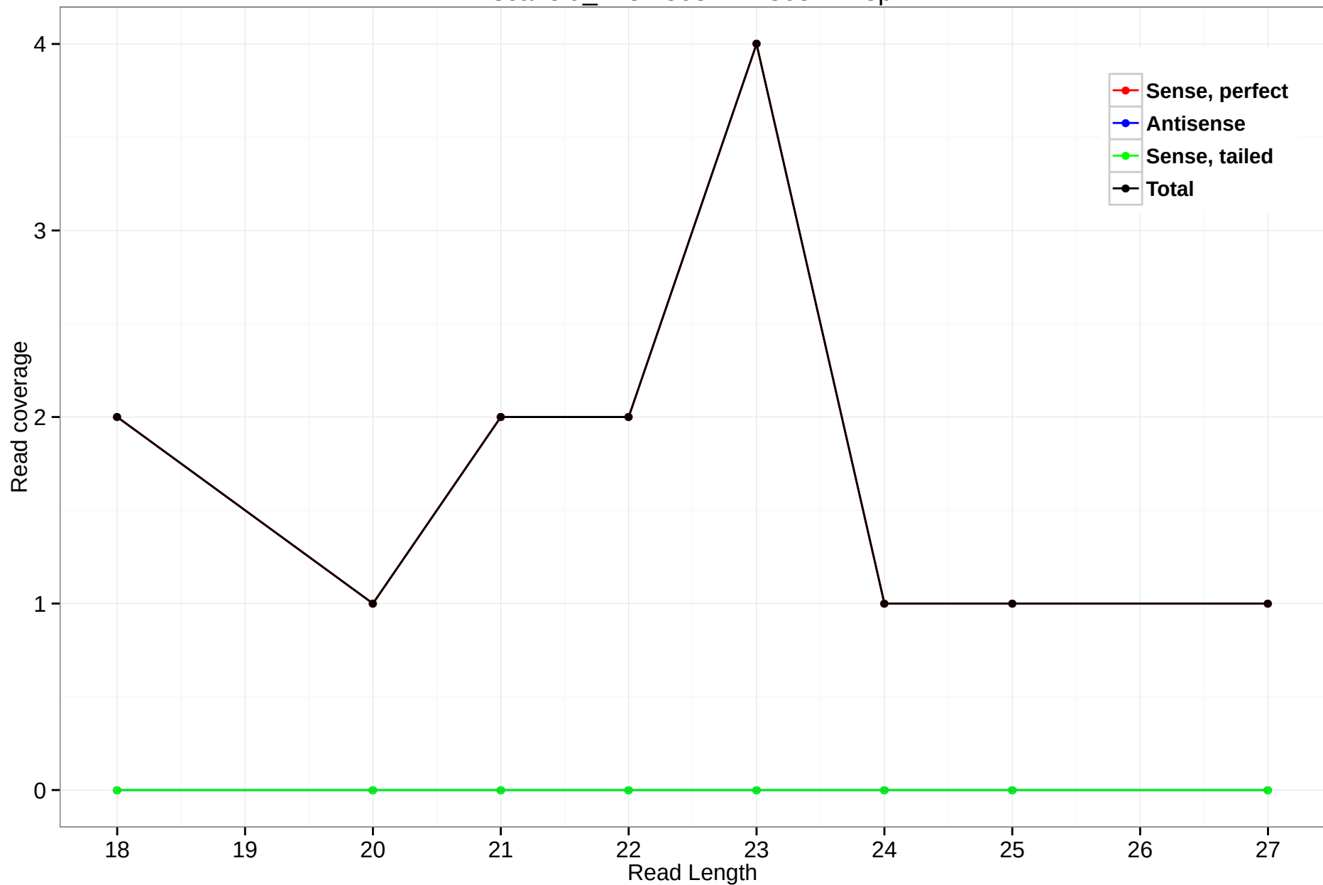
scaffold_4784:303744-305447.3p
