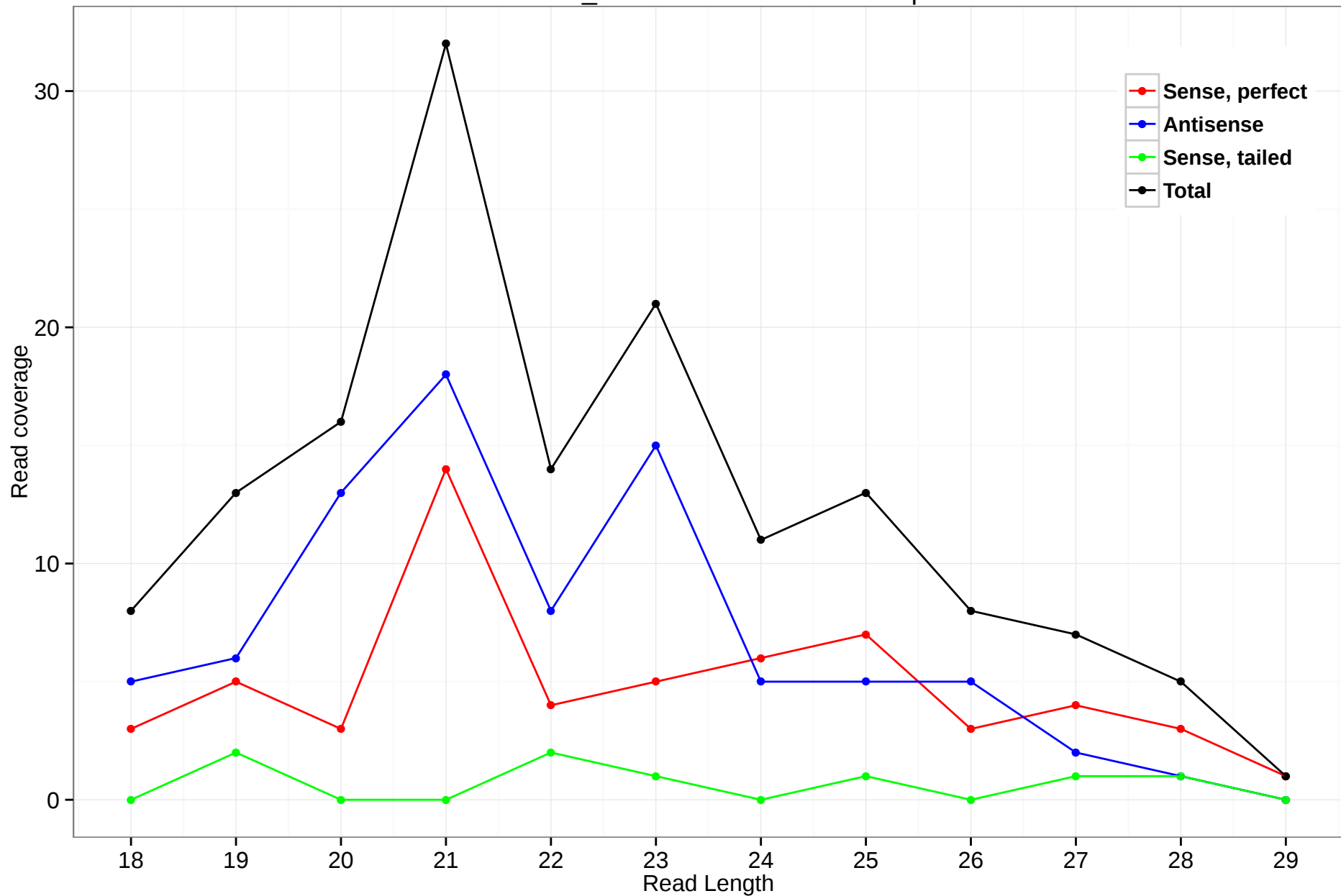
scaffold_4784:2911155-2915630.5p
