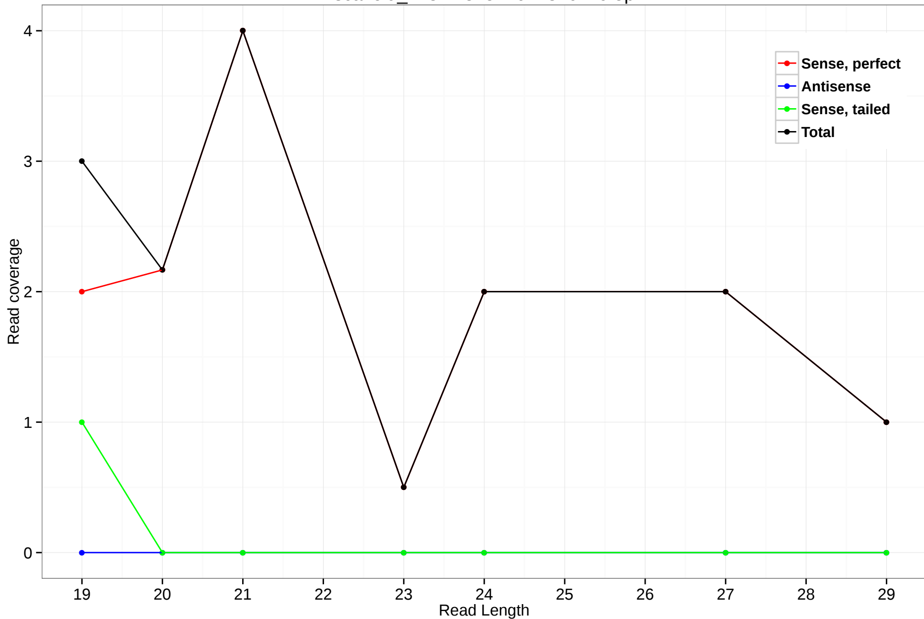
scaffold_4784:2845746-2846479.5p
