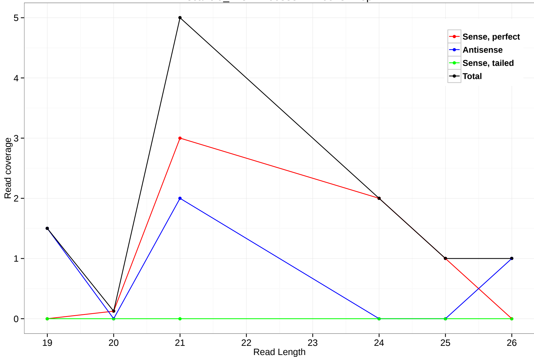
scaffold_4784:22663552-22664341.5p
