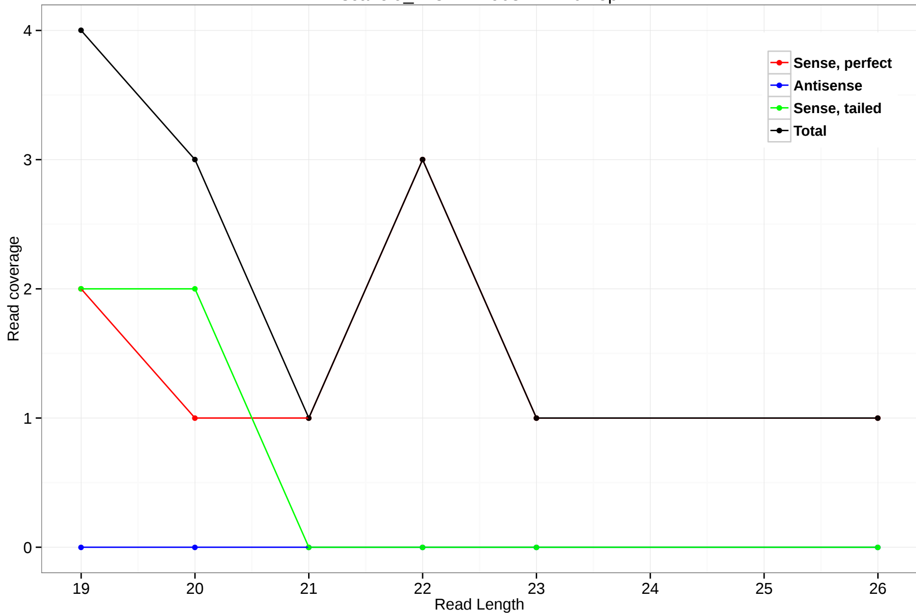
scaffold_4784:224908-227707.5p
