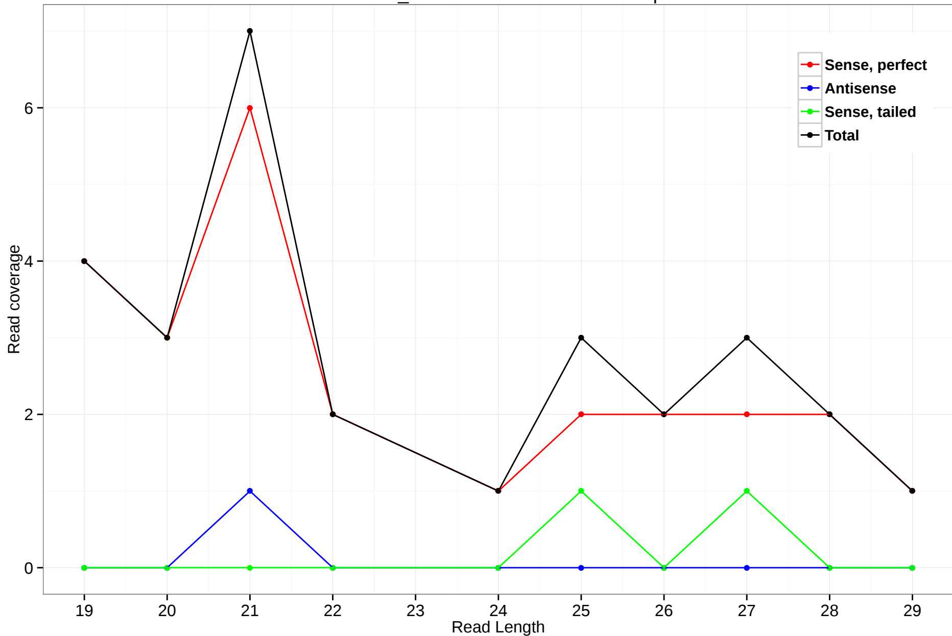
scaffold_4784:21174326-21175050.5p
