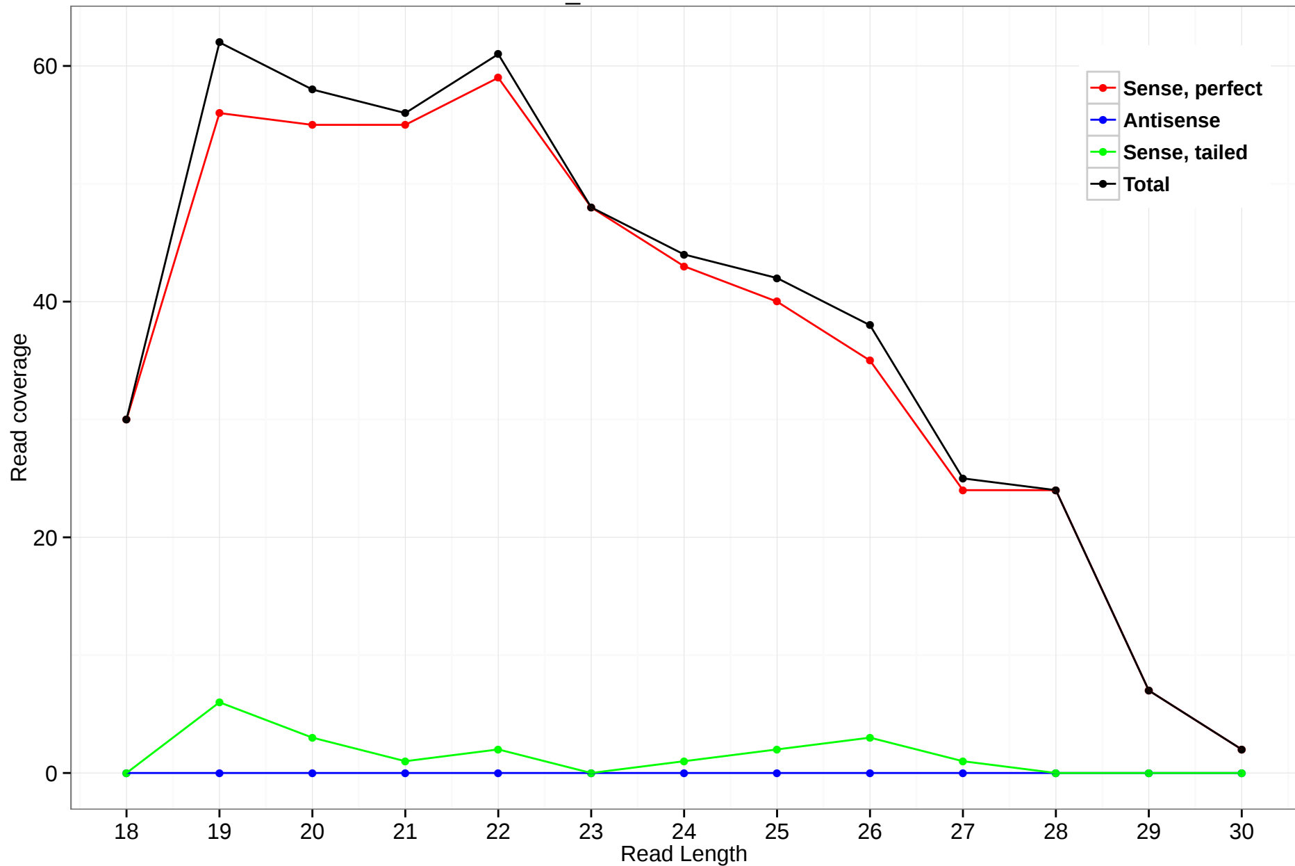
scaffold_4784:18708978-18709267
