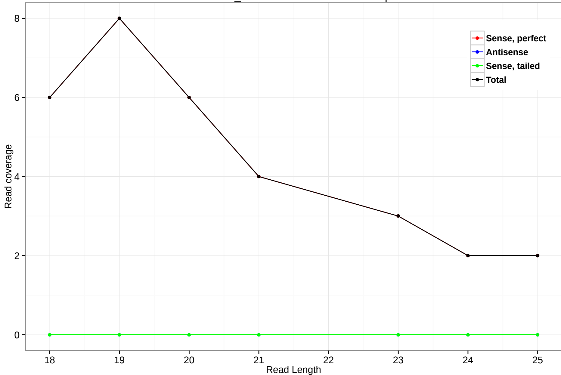
scaffold_4784:17337242-17342729.3p
