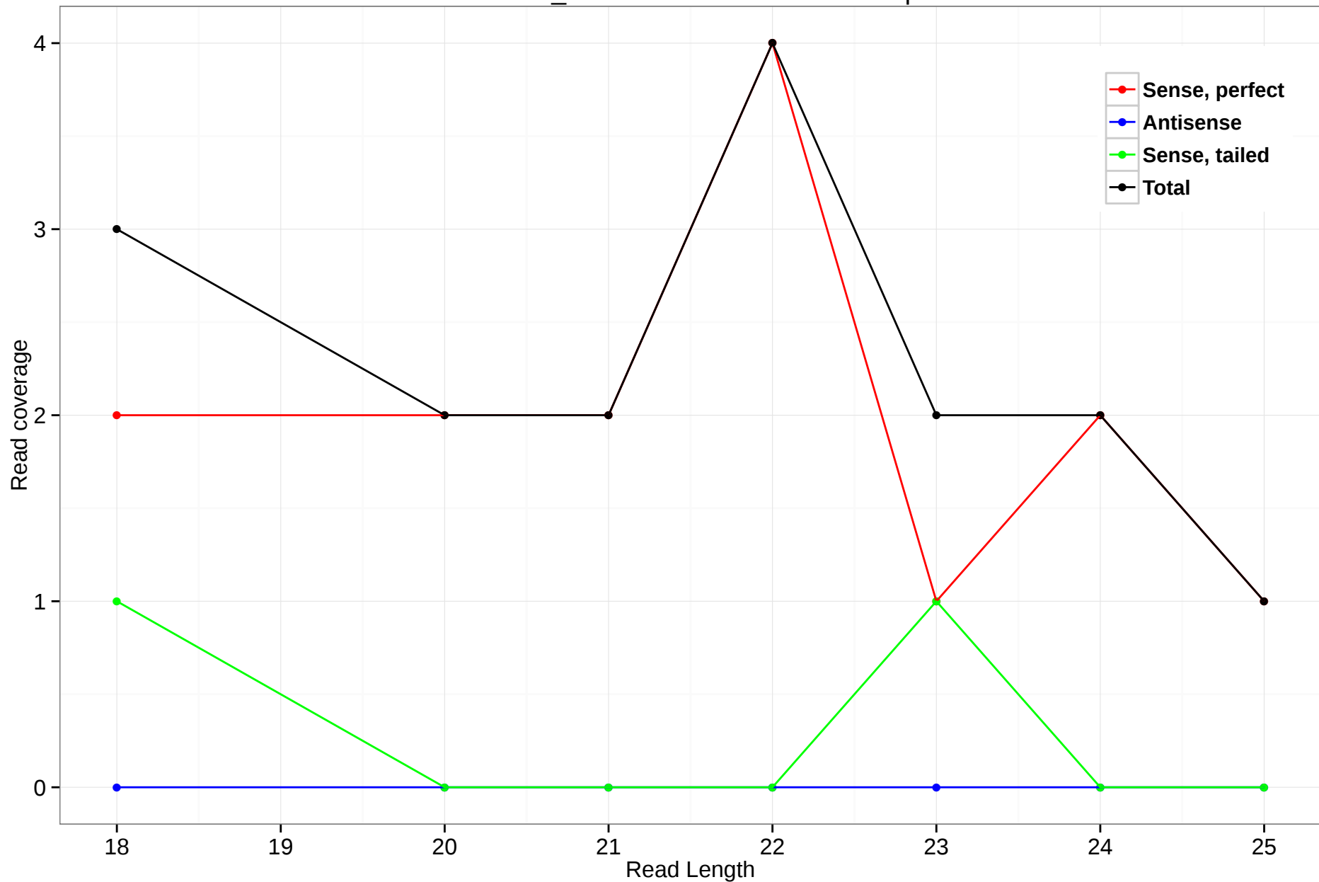
scaffold_4784:17173874-17176063.5p
