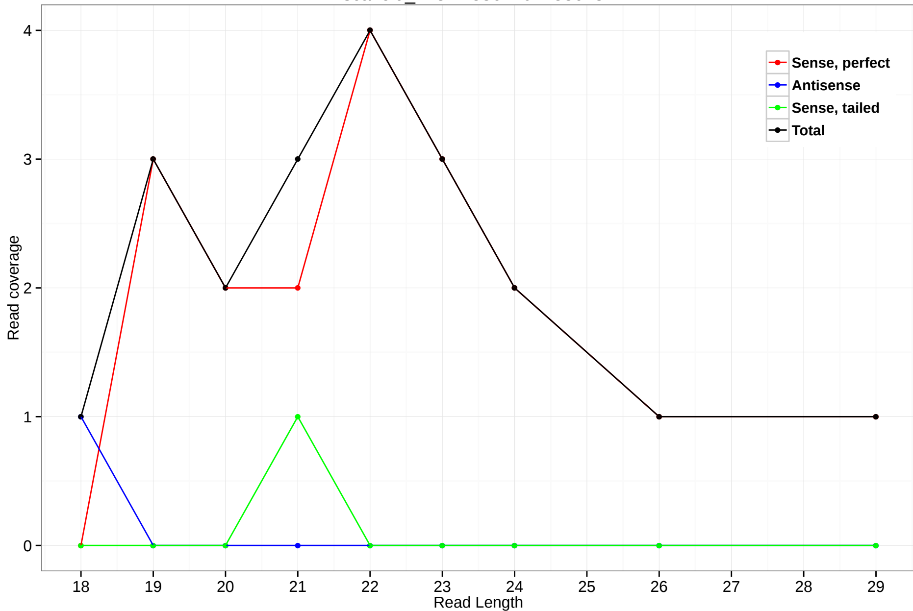
scaffold_4784:1536220-1536437
