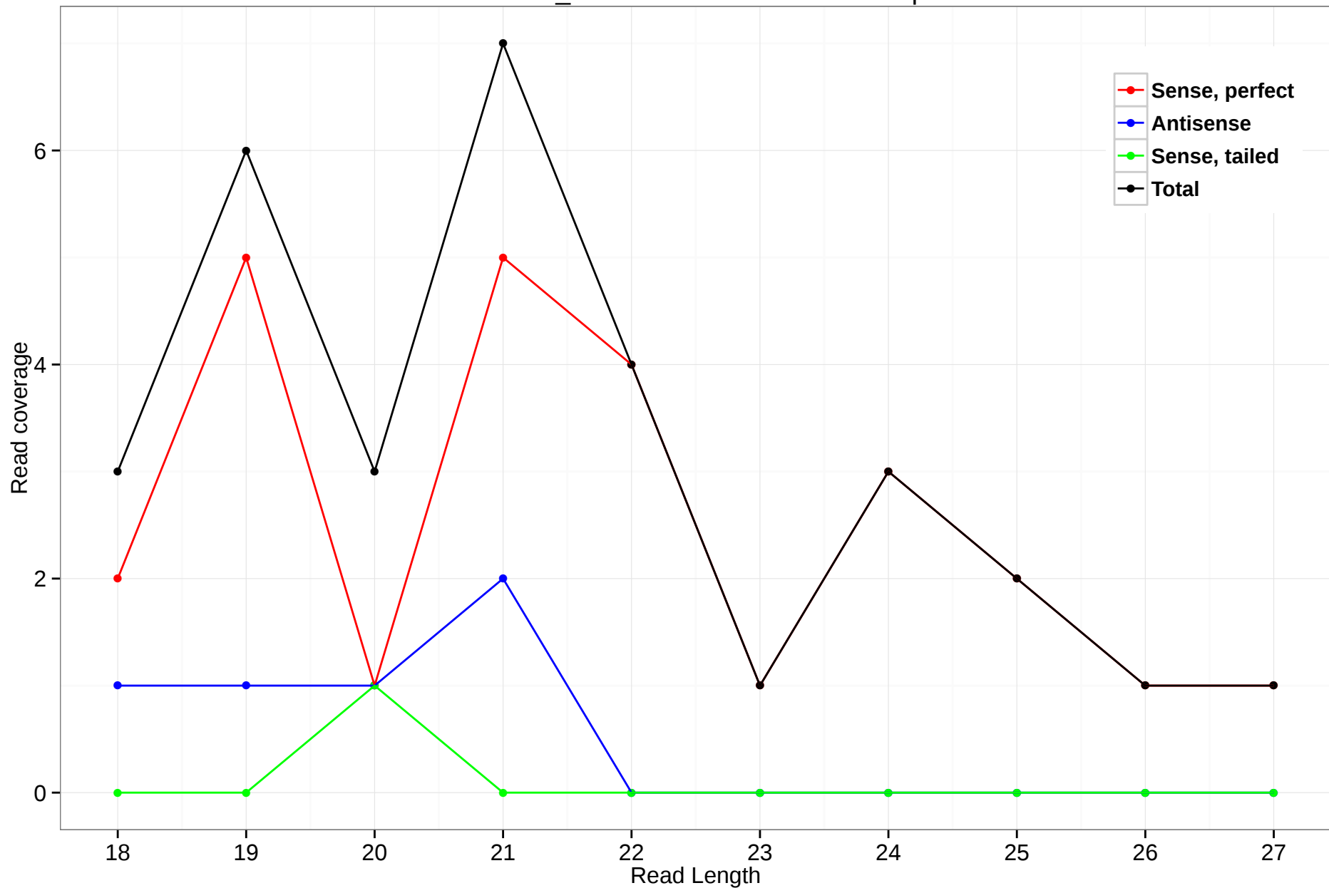
scaffold_4784:15060164-15061002.3p
