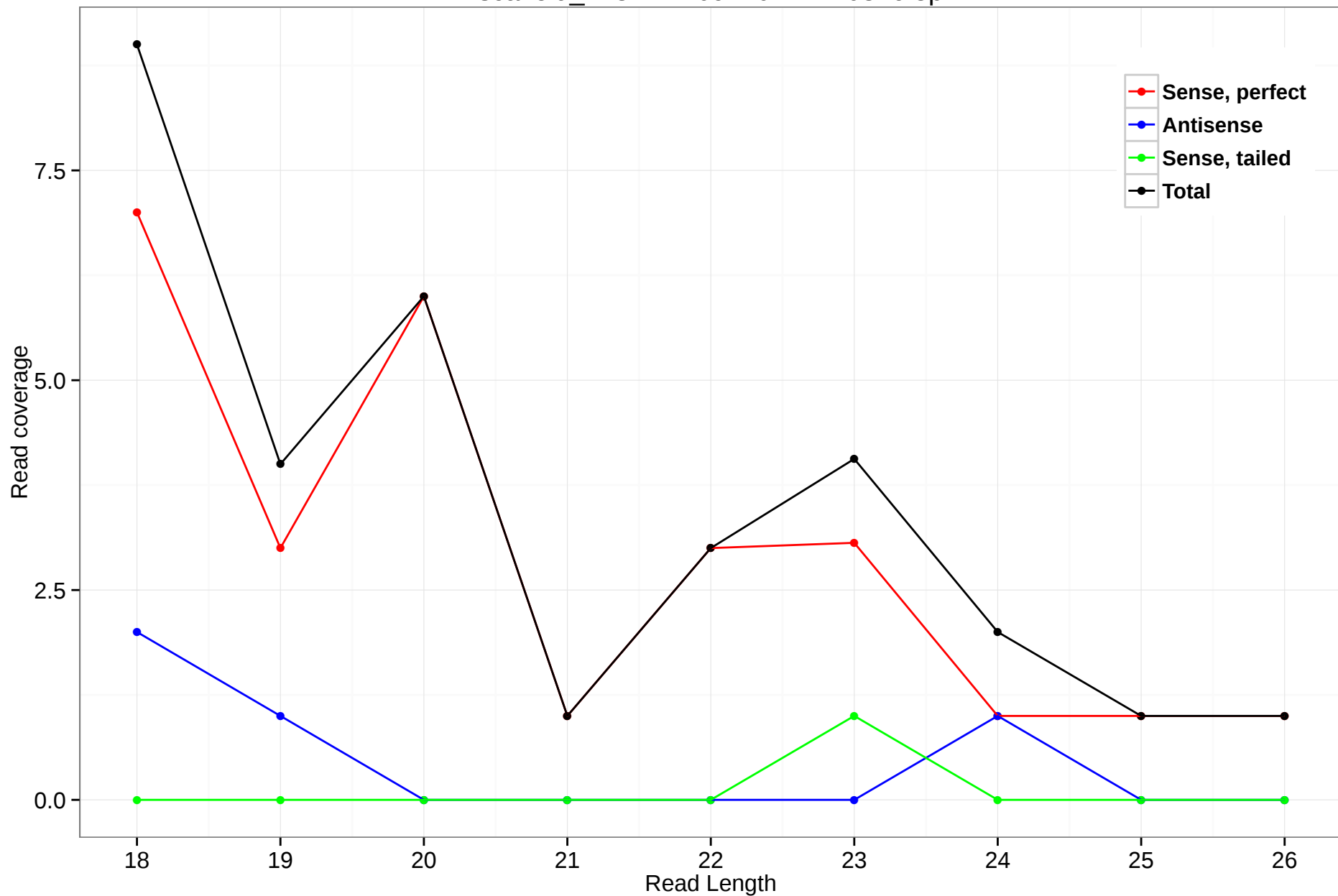
scaffold_4784:14709270-14710876.5p
