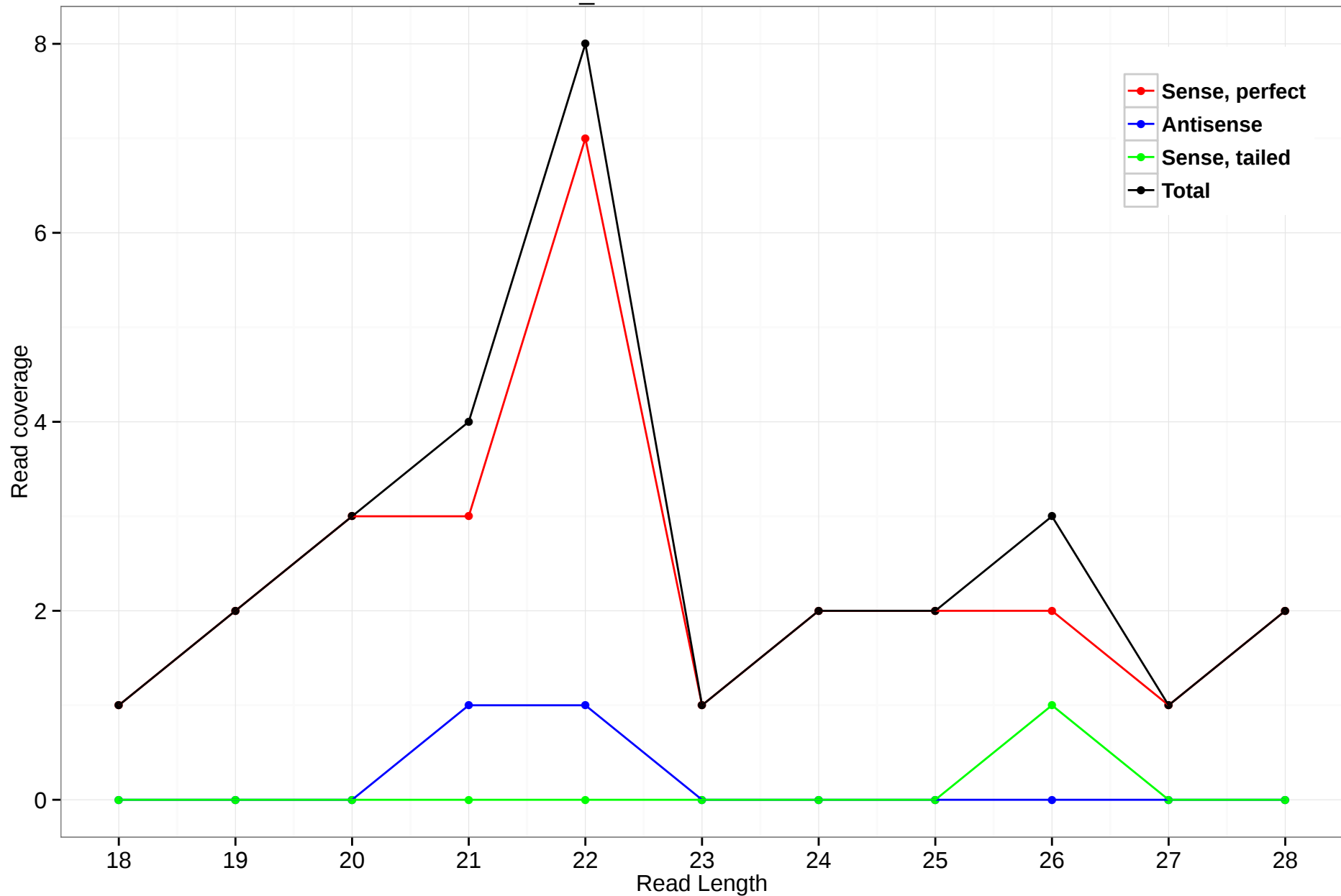
scaffold_4784:12104950-12105473
