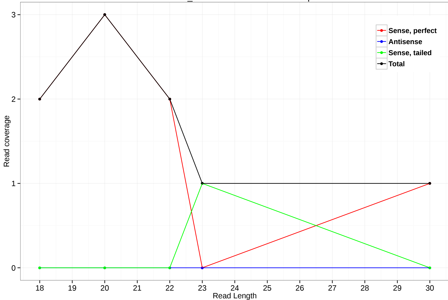
scaffold_4784:11491227-11491844.5p
