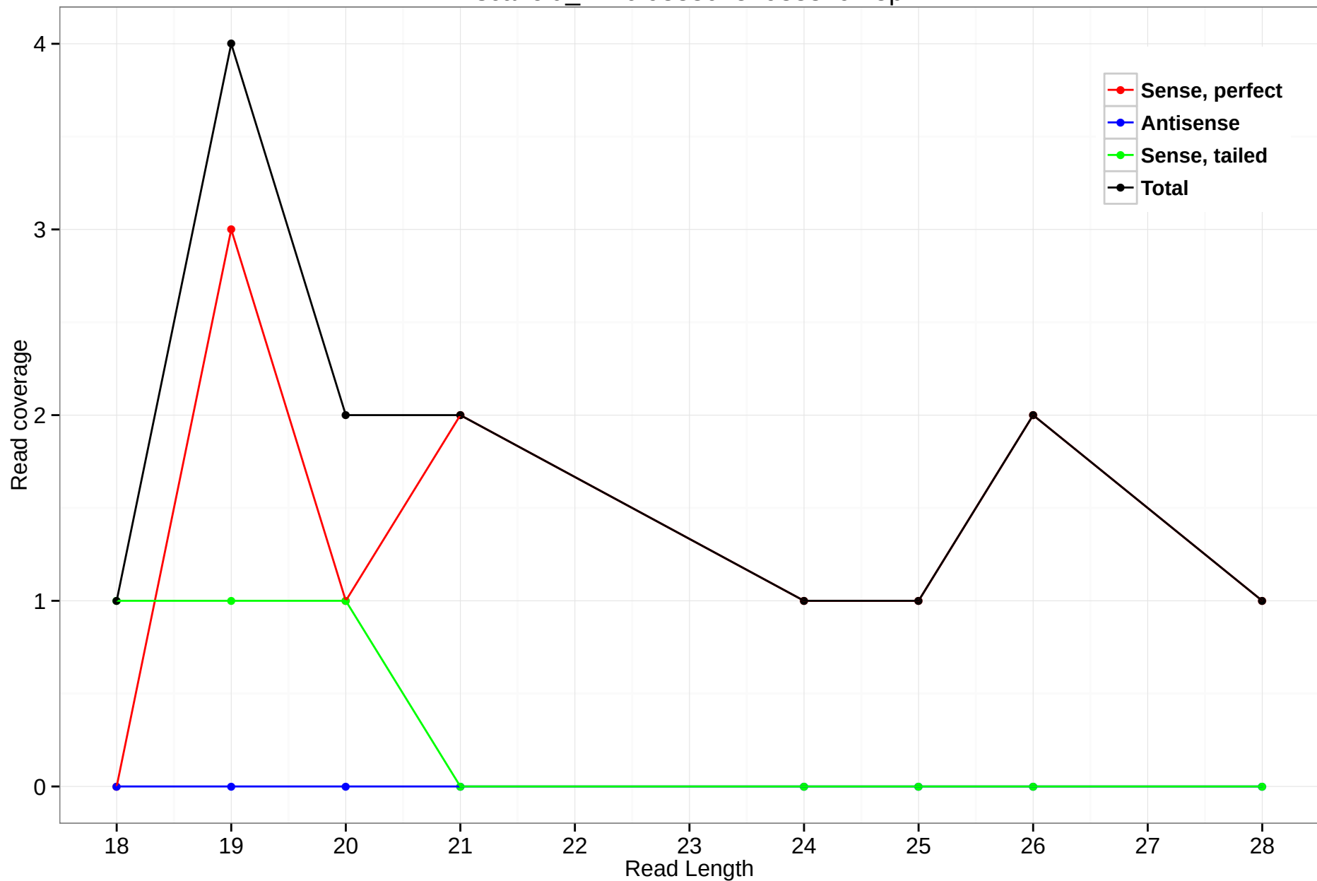
scaffold_4770:9838075-9838797.5p
