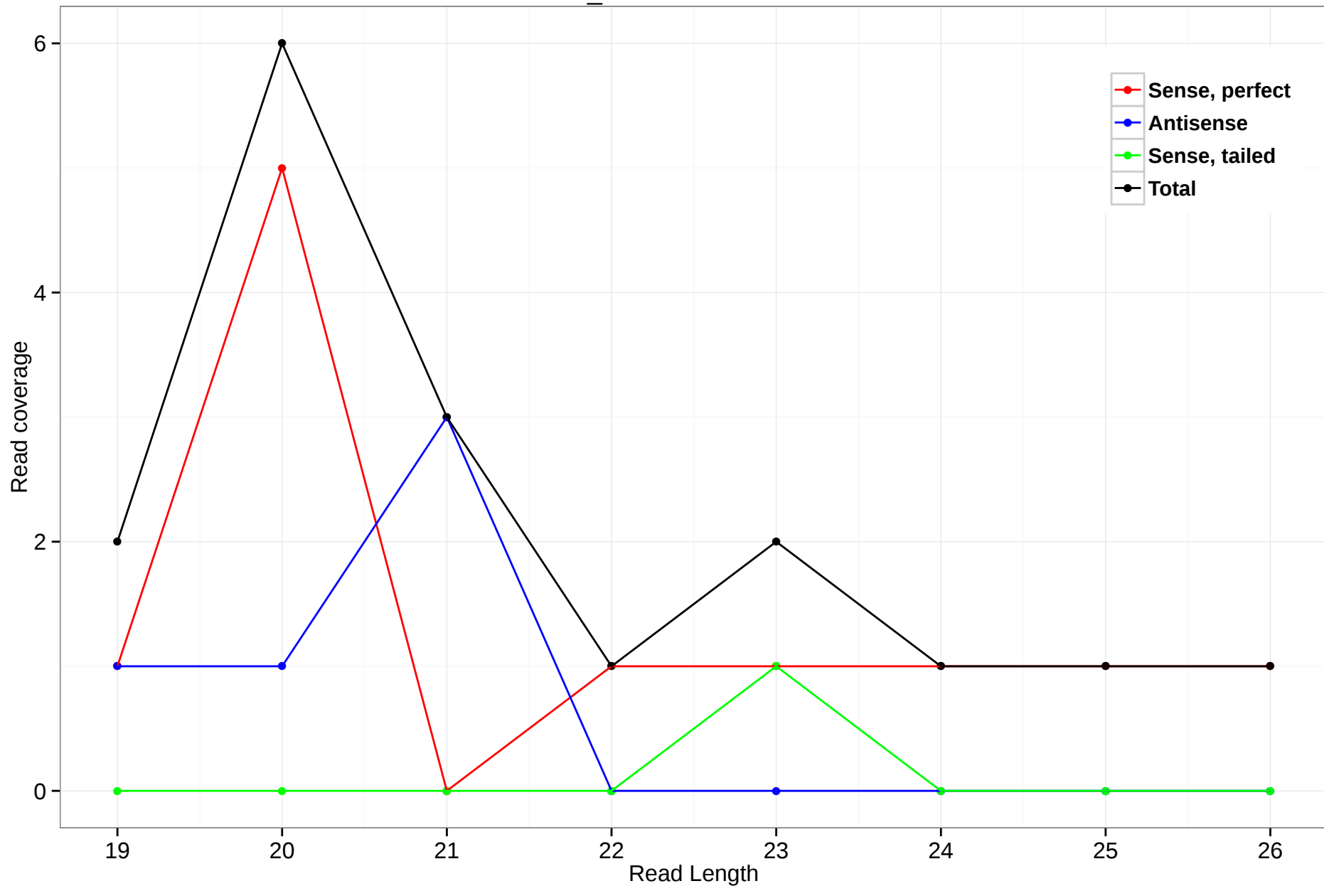
scaffold_4770:9401318-9401633
