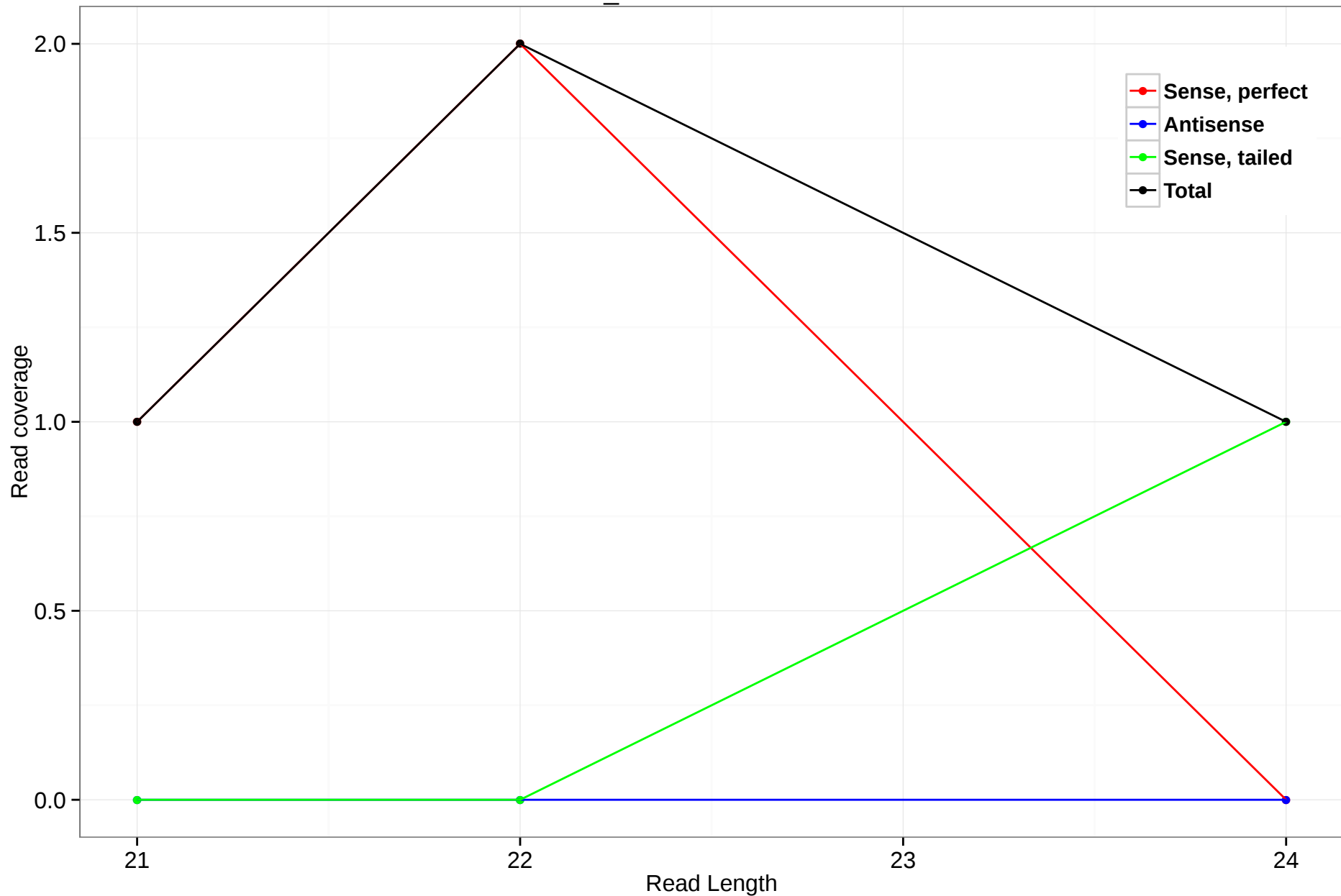
scaffold_4770:9192981-9193136
