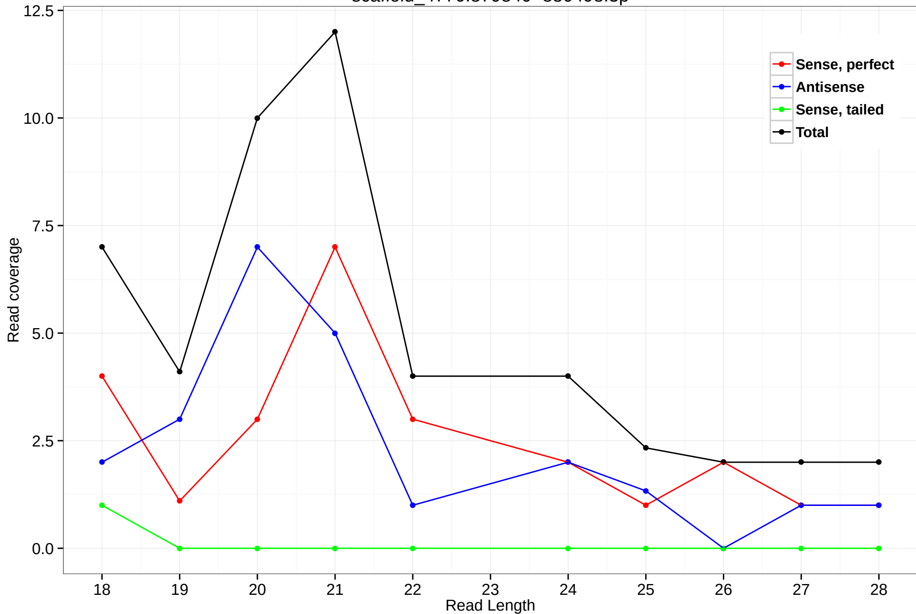
scaffold_4770:879840-880498.3p
