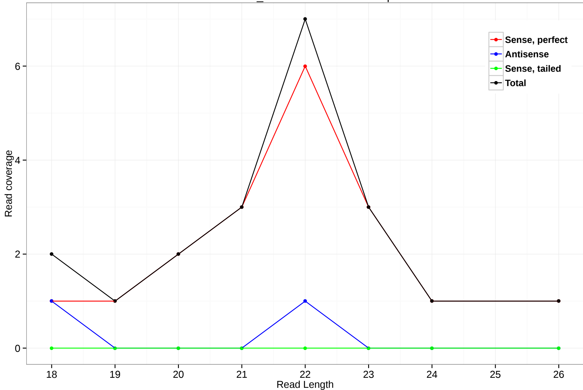
scaffold_4770:792115-793058.5p
