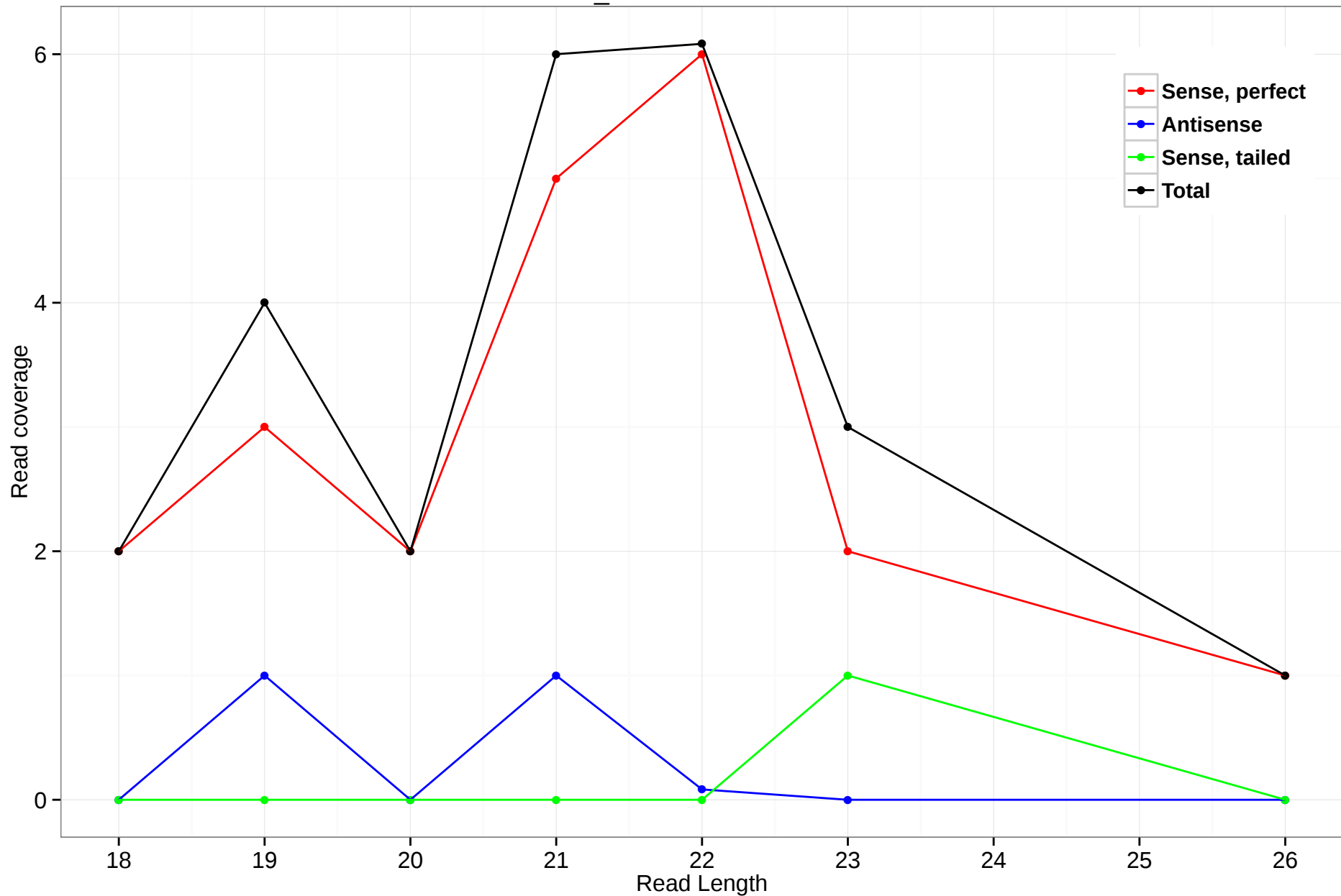
scaffold_4770:6579851-6580360
