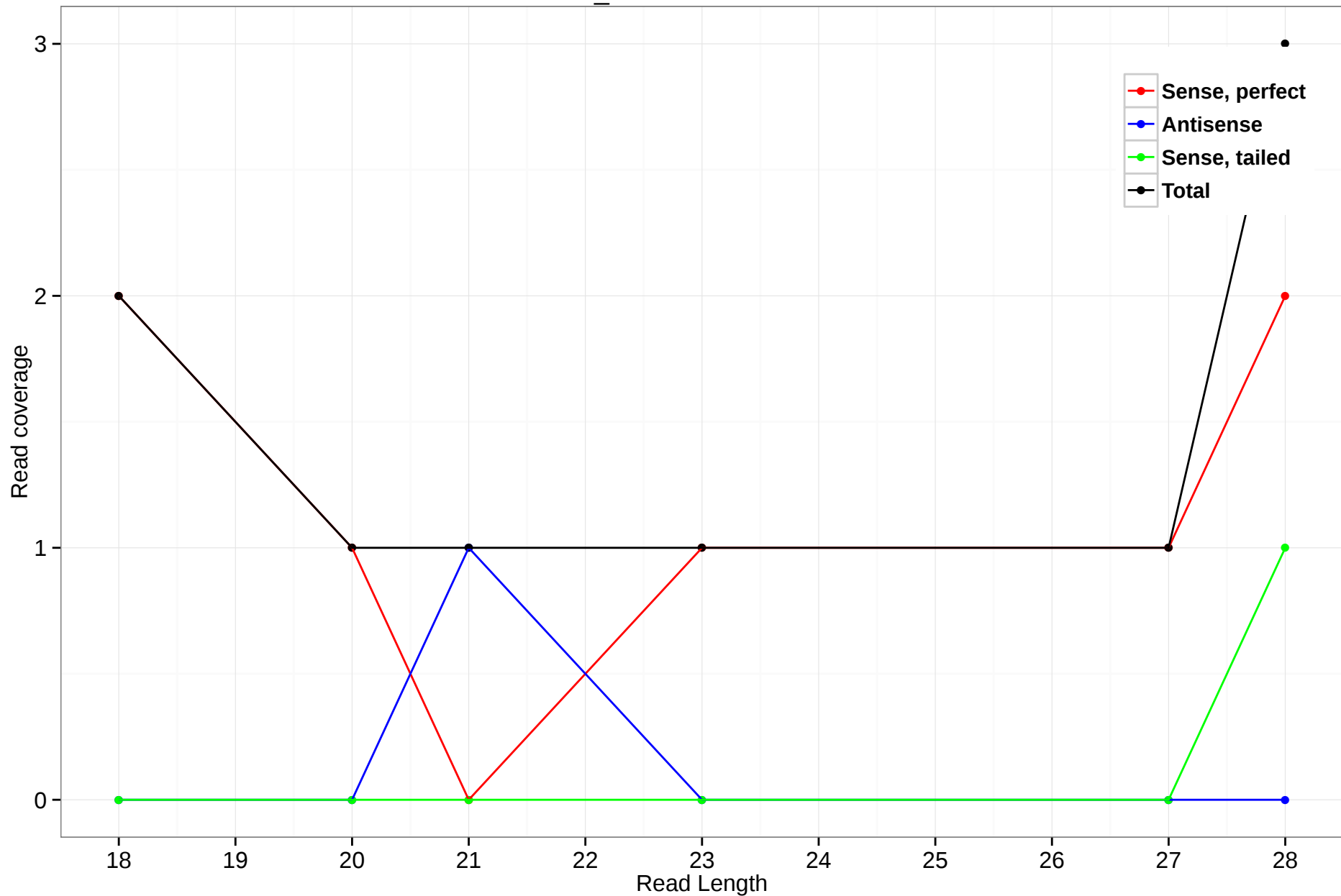
scaffold_4770:6223559-6223850
