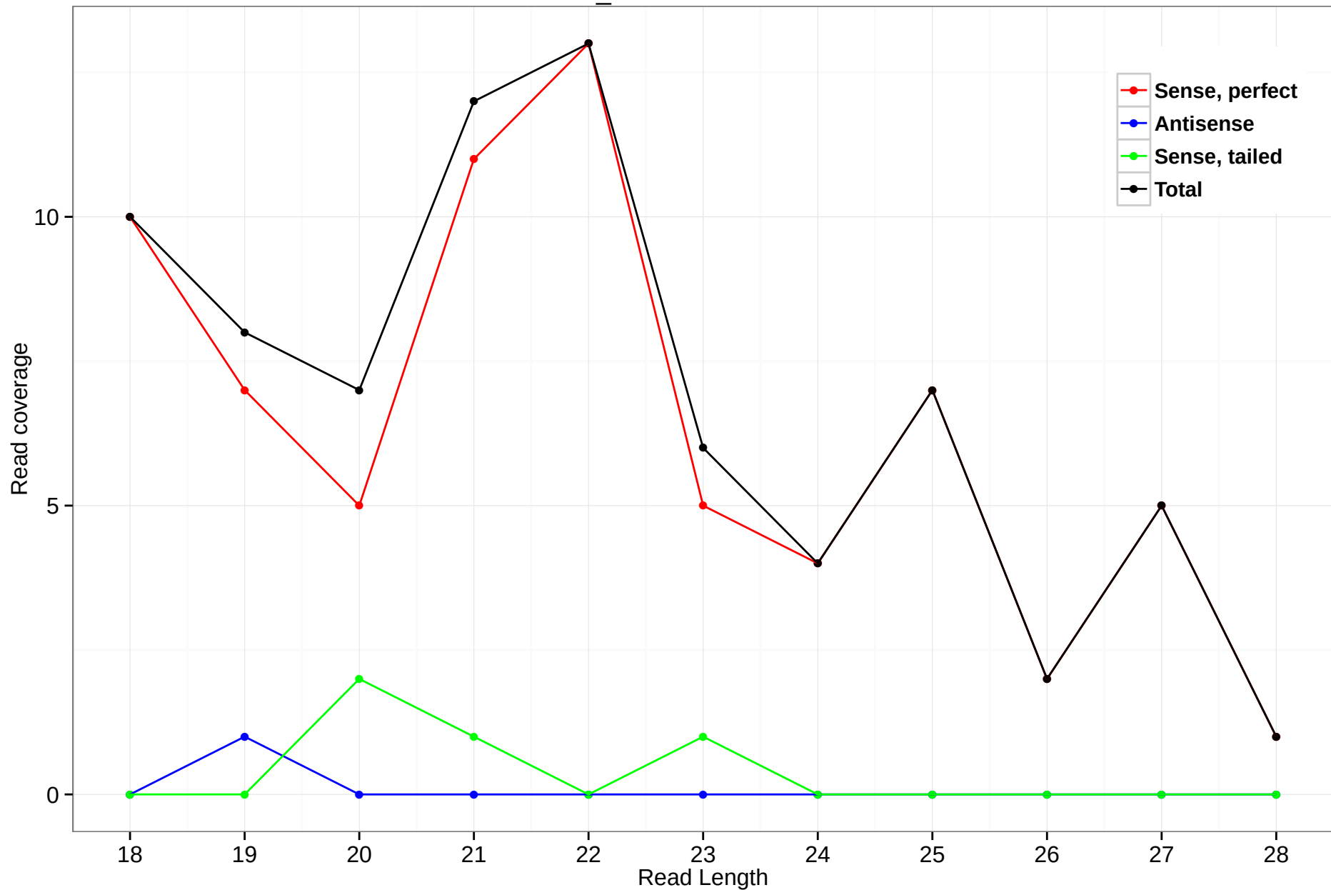
scaffold_4770:6171244-6171711
