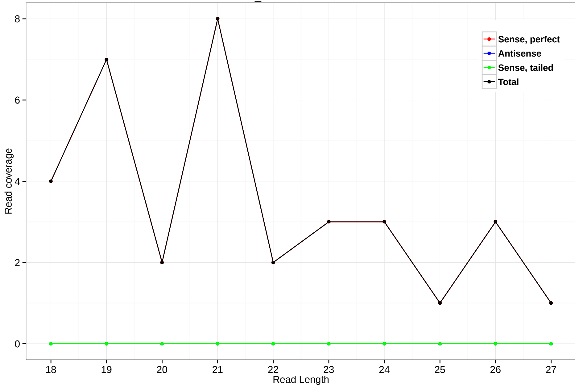
scaffold_4770:5937542-5937923
