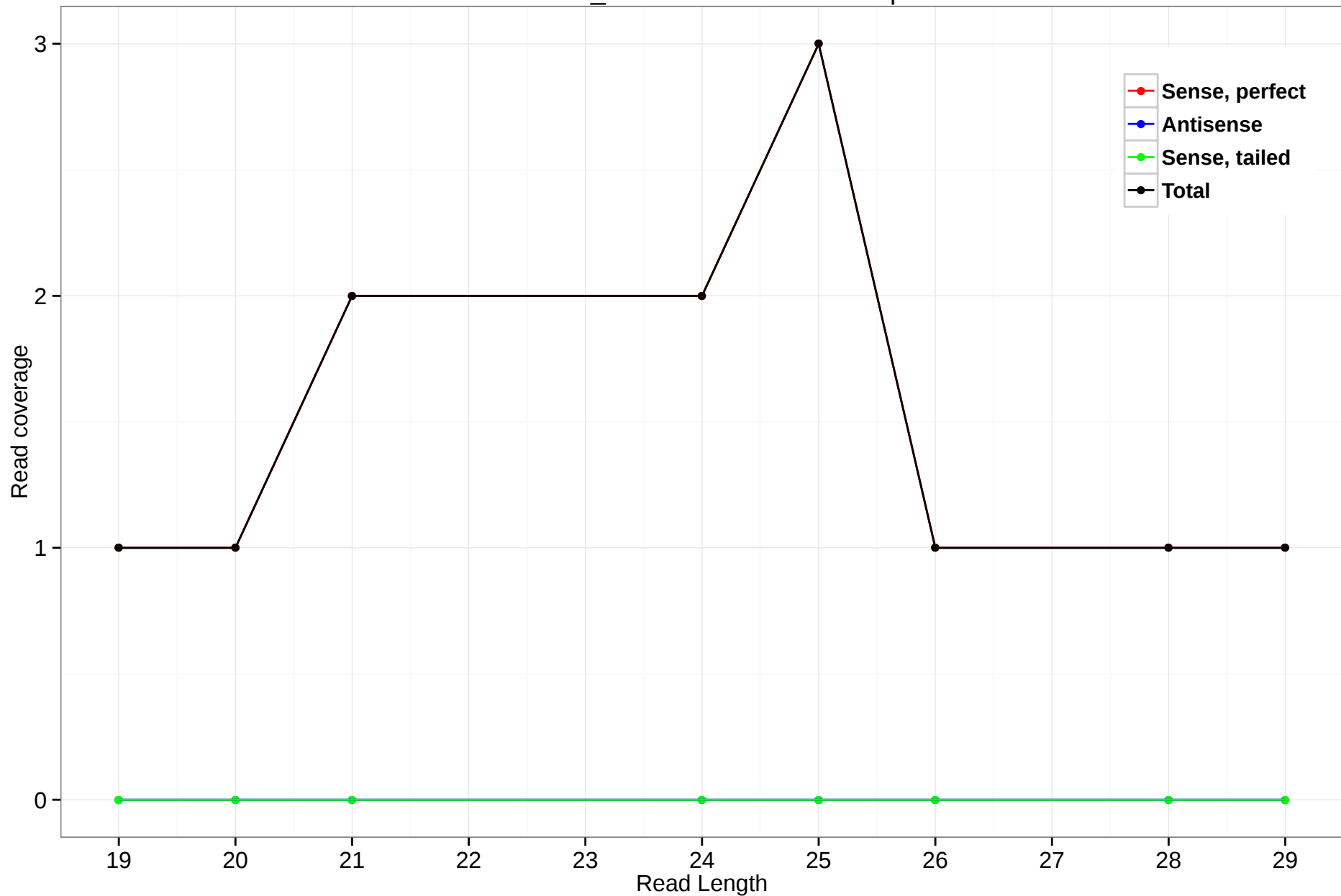
scaffold_4770:565366-567958.5p
