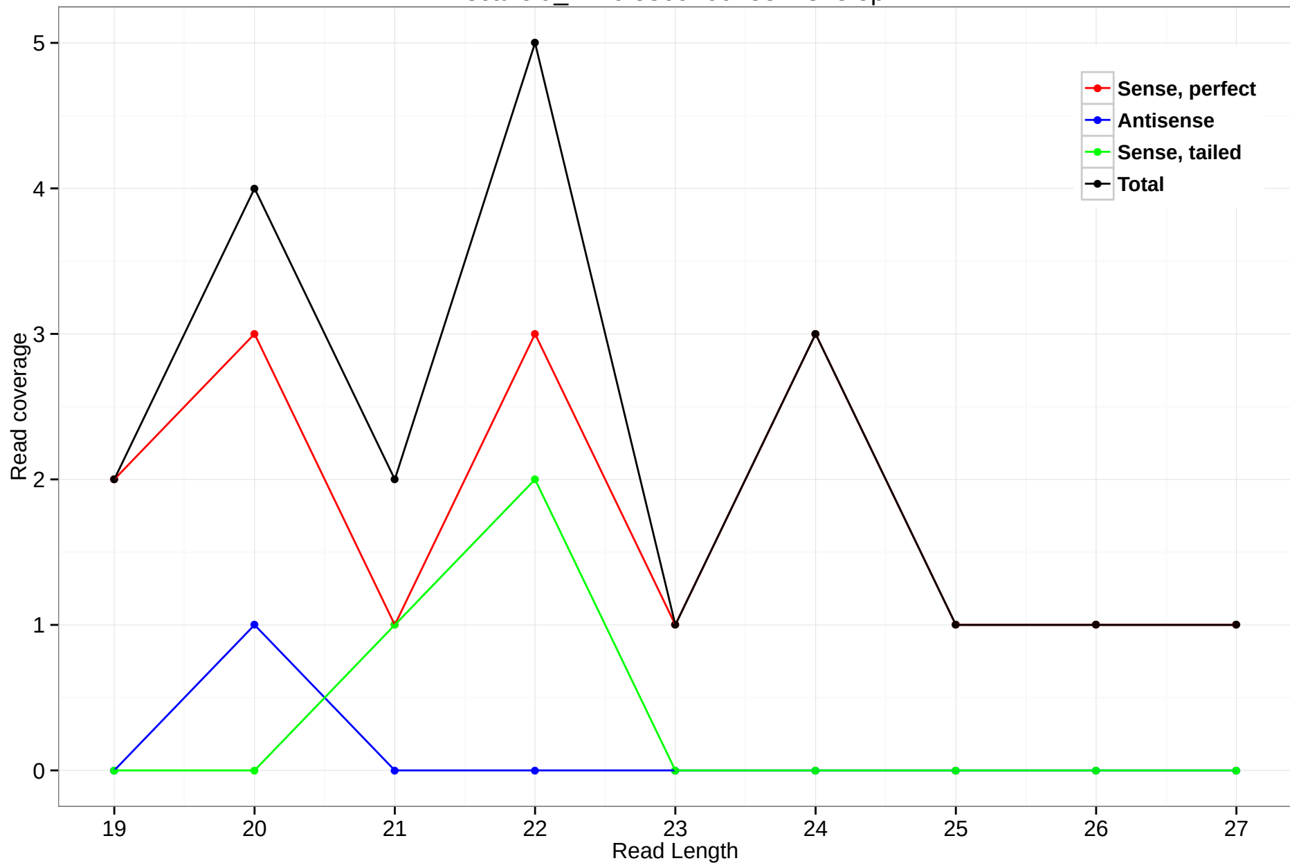
scaffold_4770:5309460-5311313.5p
