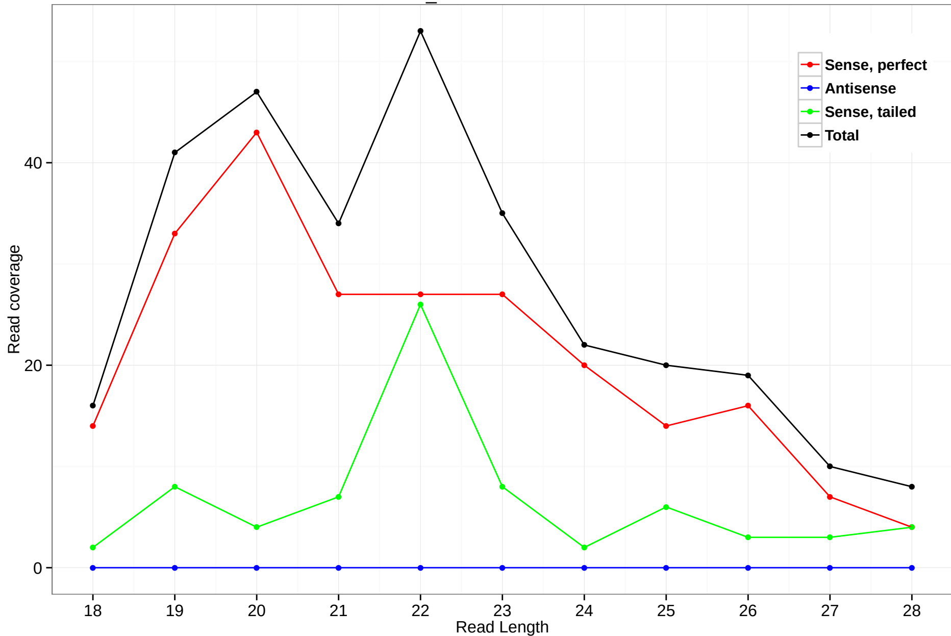
scaffold_4770:5014325-5014685
