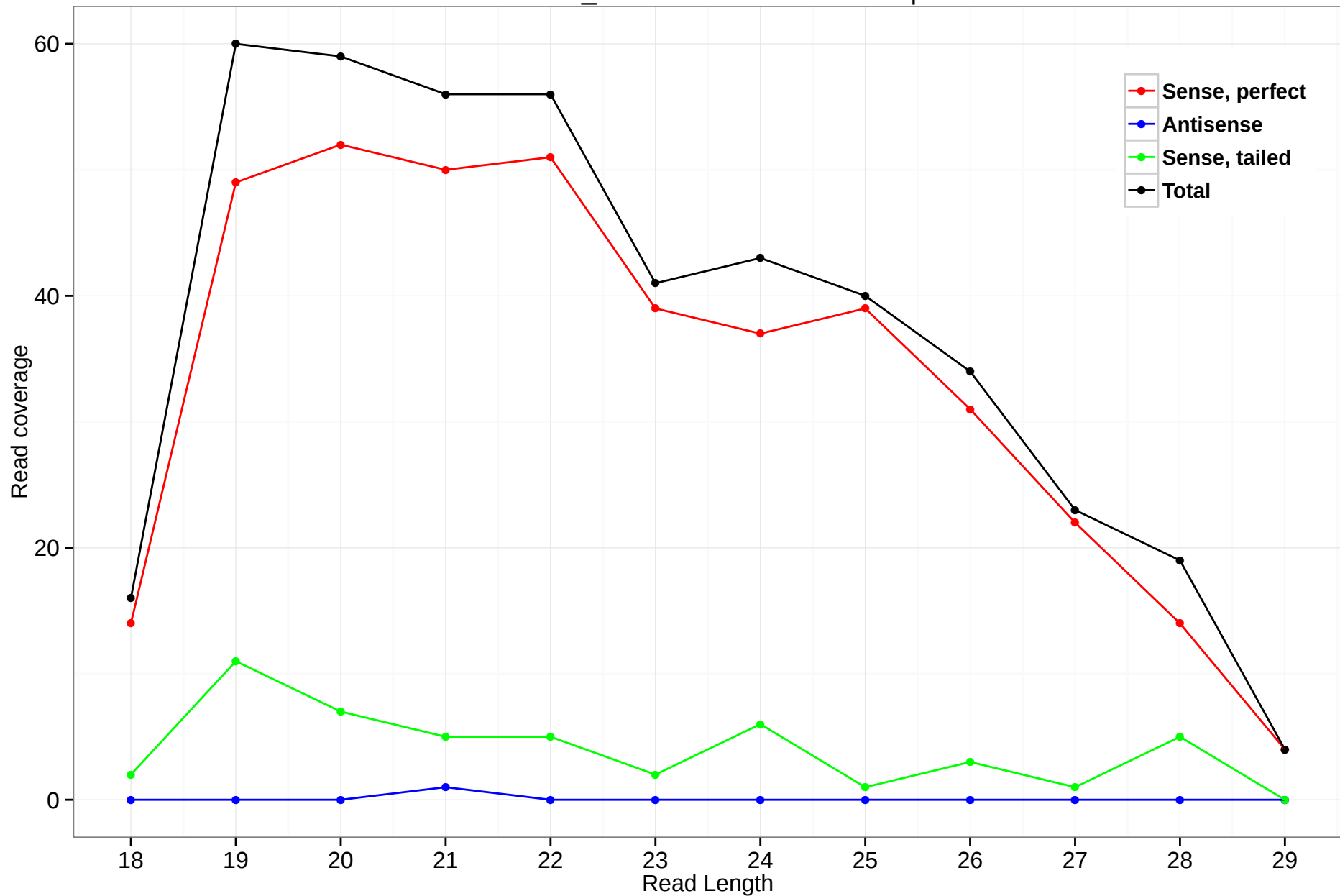
scaffold_4770:4901241-4918978.3p
