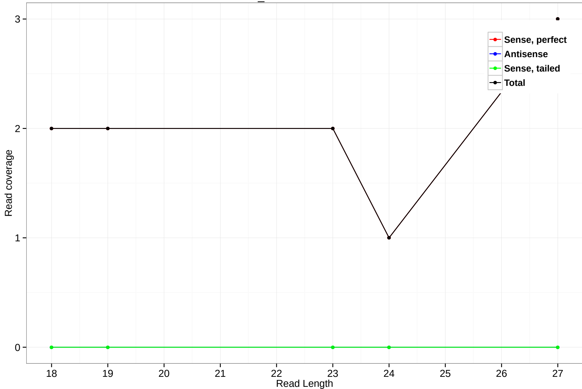
scaffold_4770:4852498-4852802
