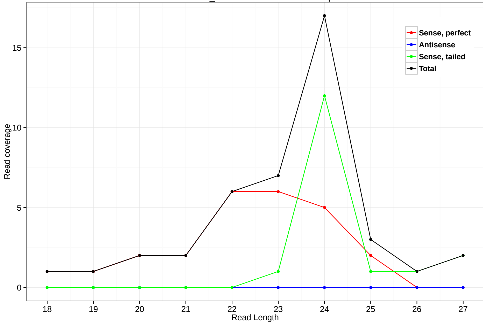
scaffold_4770:4216871-4218064.5p
