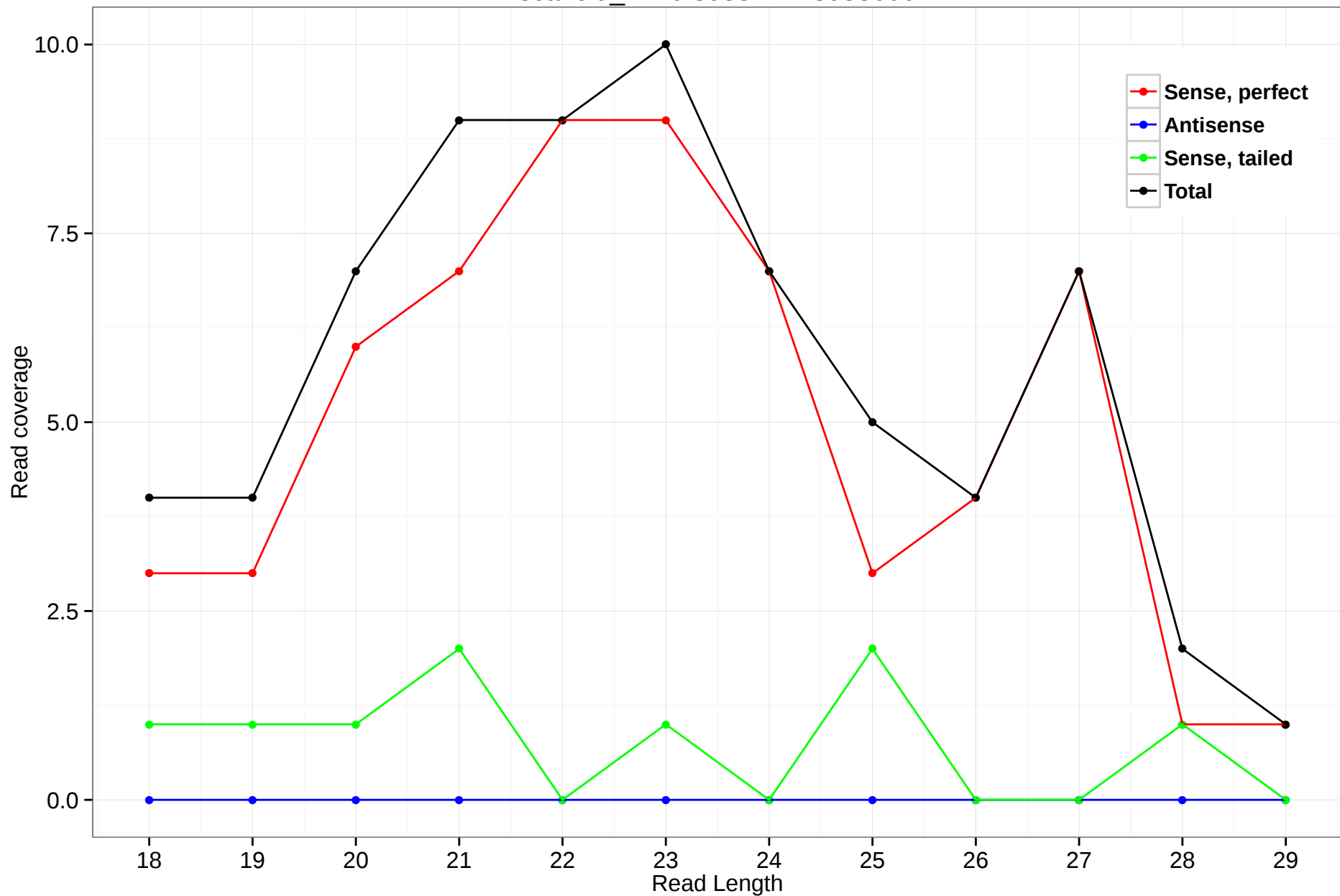
scaffold_4770:3988214-3988600
