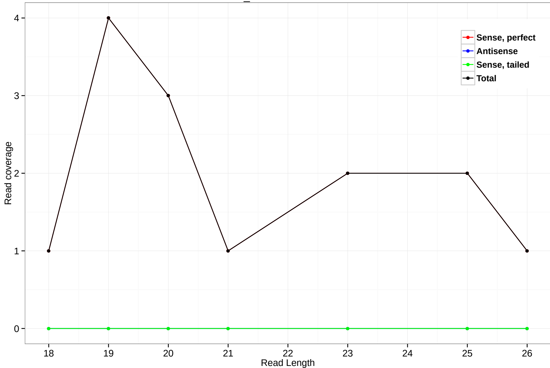
scaffold_4770:3979688-3979854
