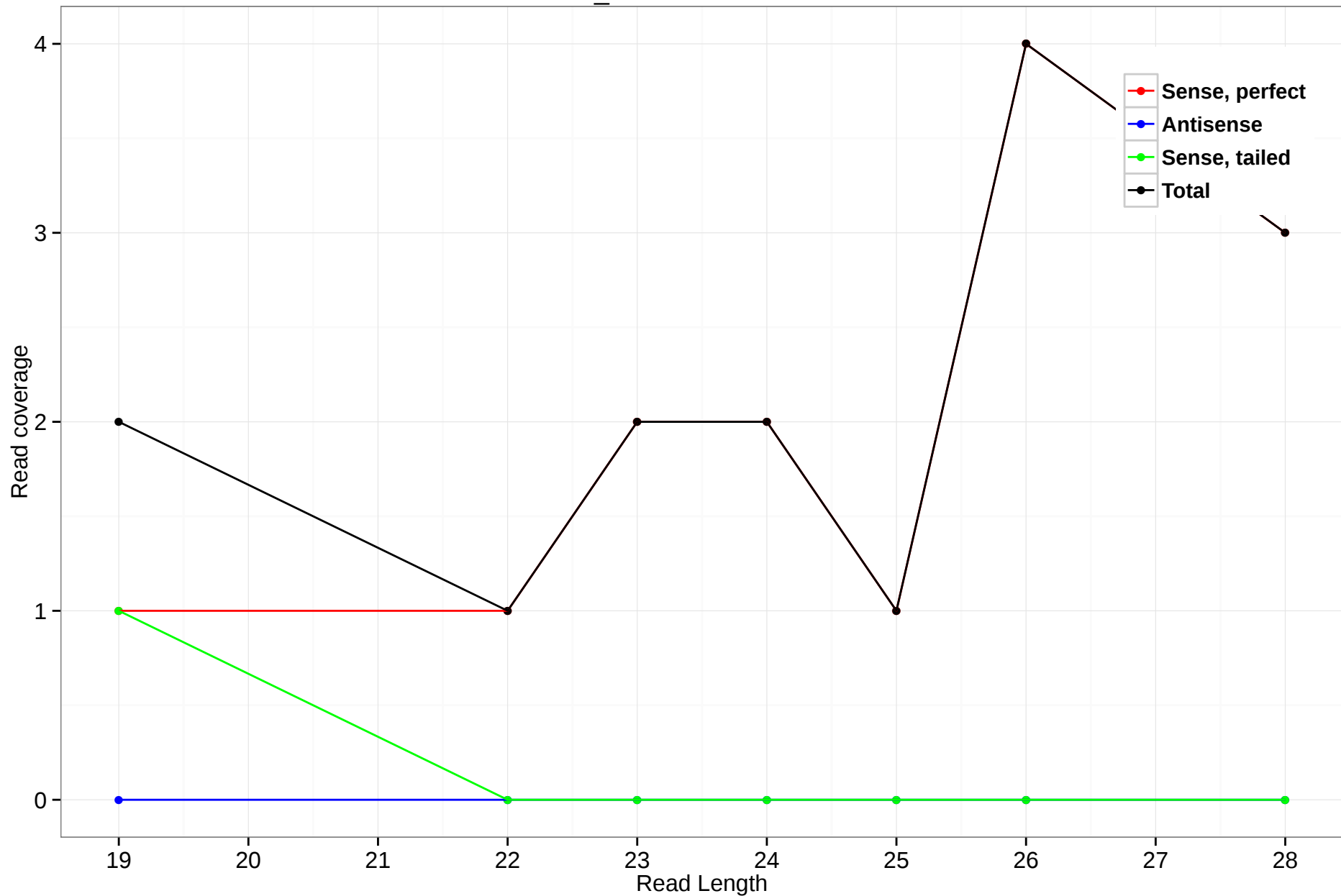
scaffold_4770:3850796-3851295
