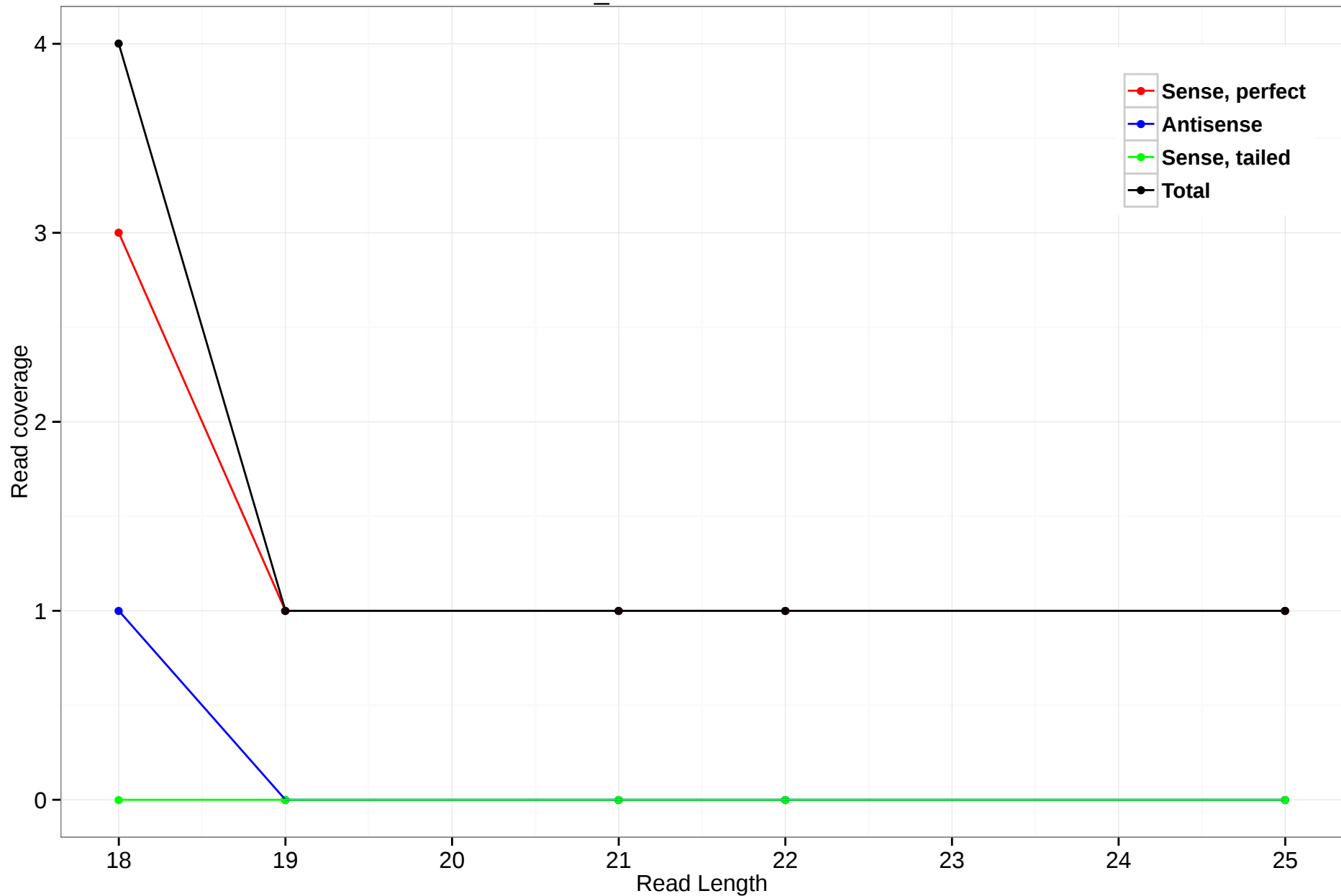
scaffold_4770:3280511-3281090
