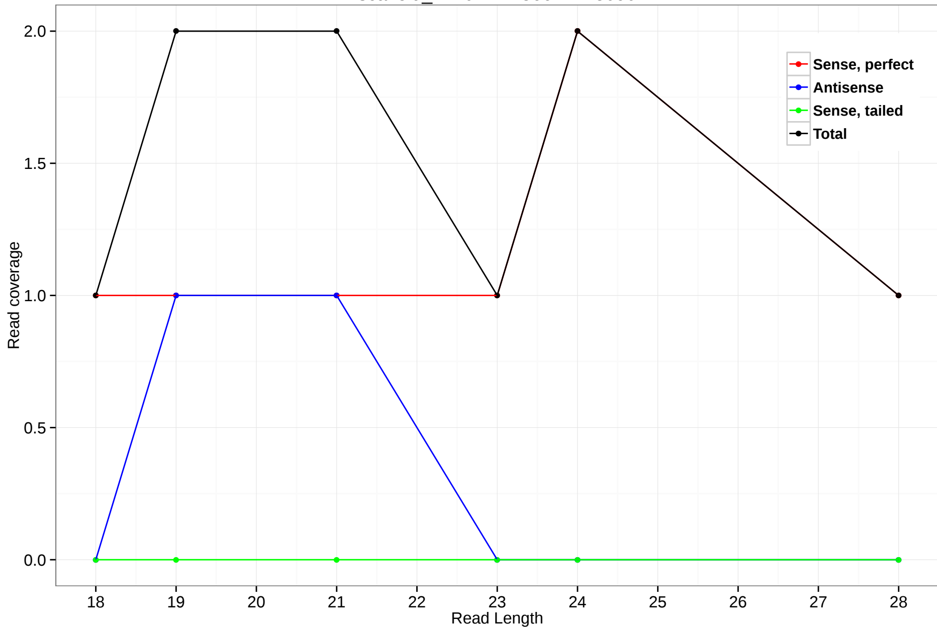
scaffold_4770:2444566-2445090
