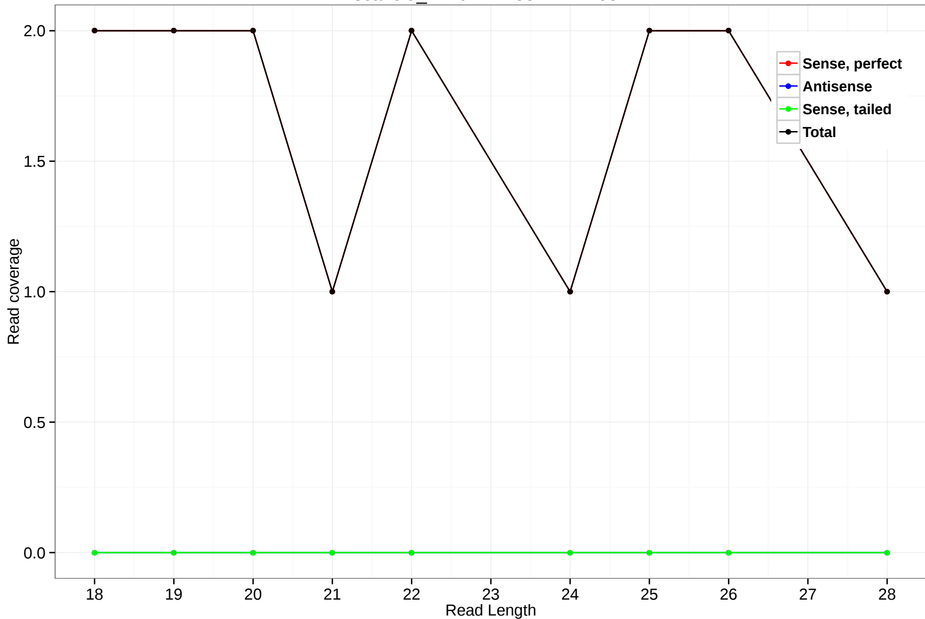
scaffold_4770:1747382-1747687
