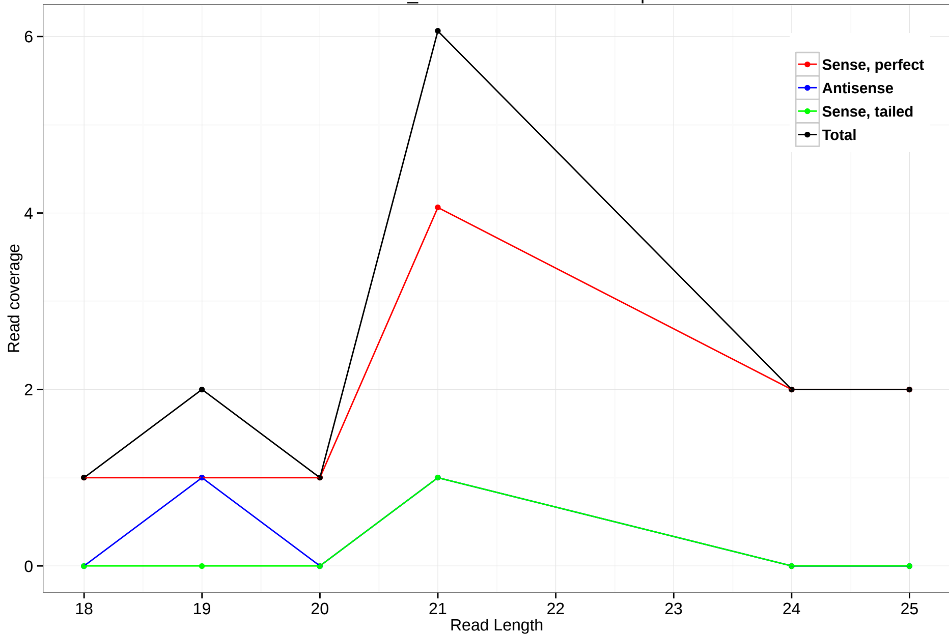
scaffold_4770:1740070-1740822.5p
