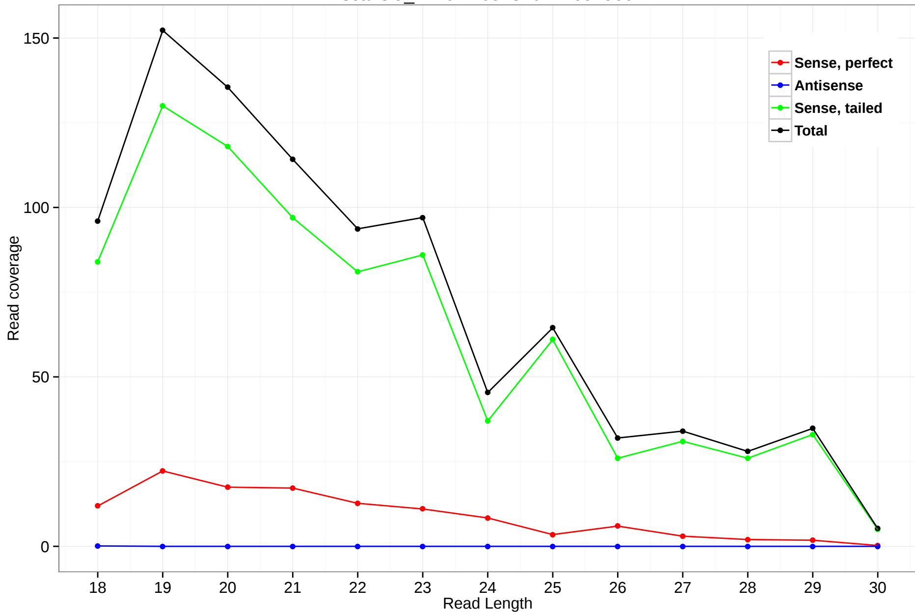
scaffold_4770:17091840-17091960
