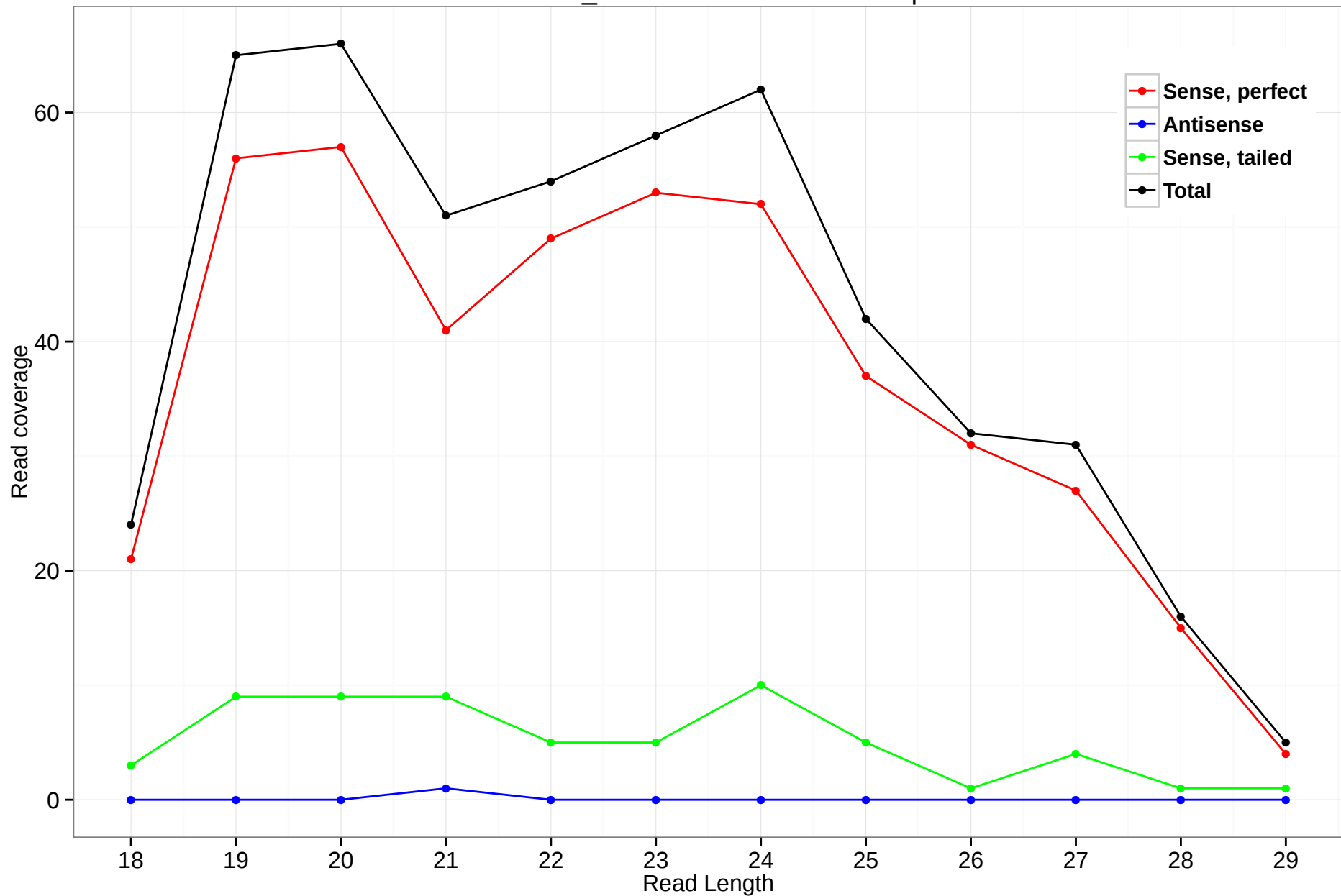
scaffold_4770:1692283-1693104.5p
