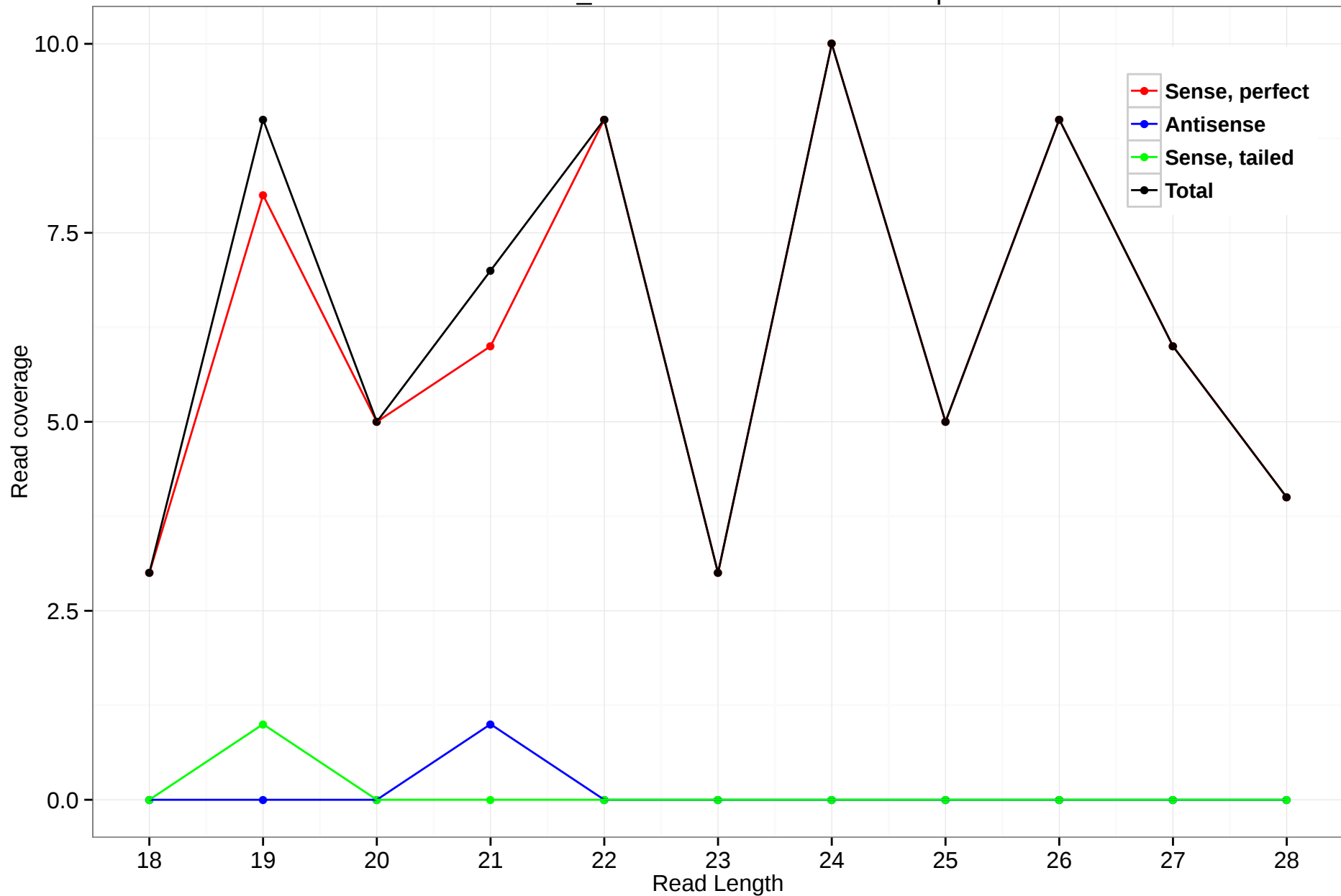
scaffold_4770:16835219-16835922.5p
